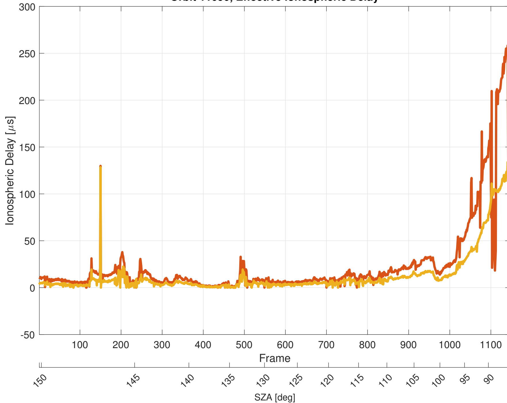
Orbit 11090, Effective Ionospheric Delay
