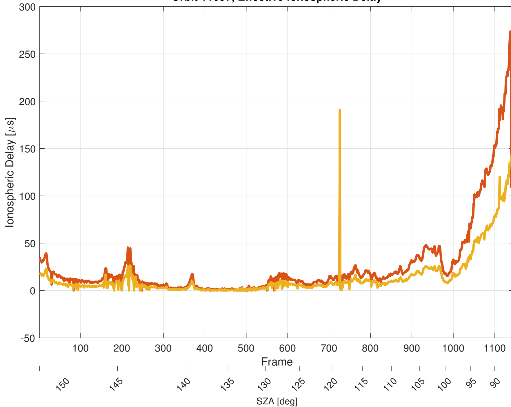
Orbit 11097, Effective Ionospheric Delay
