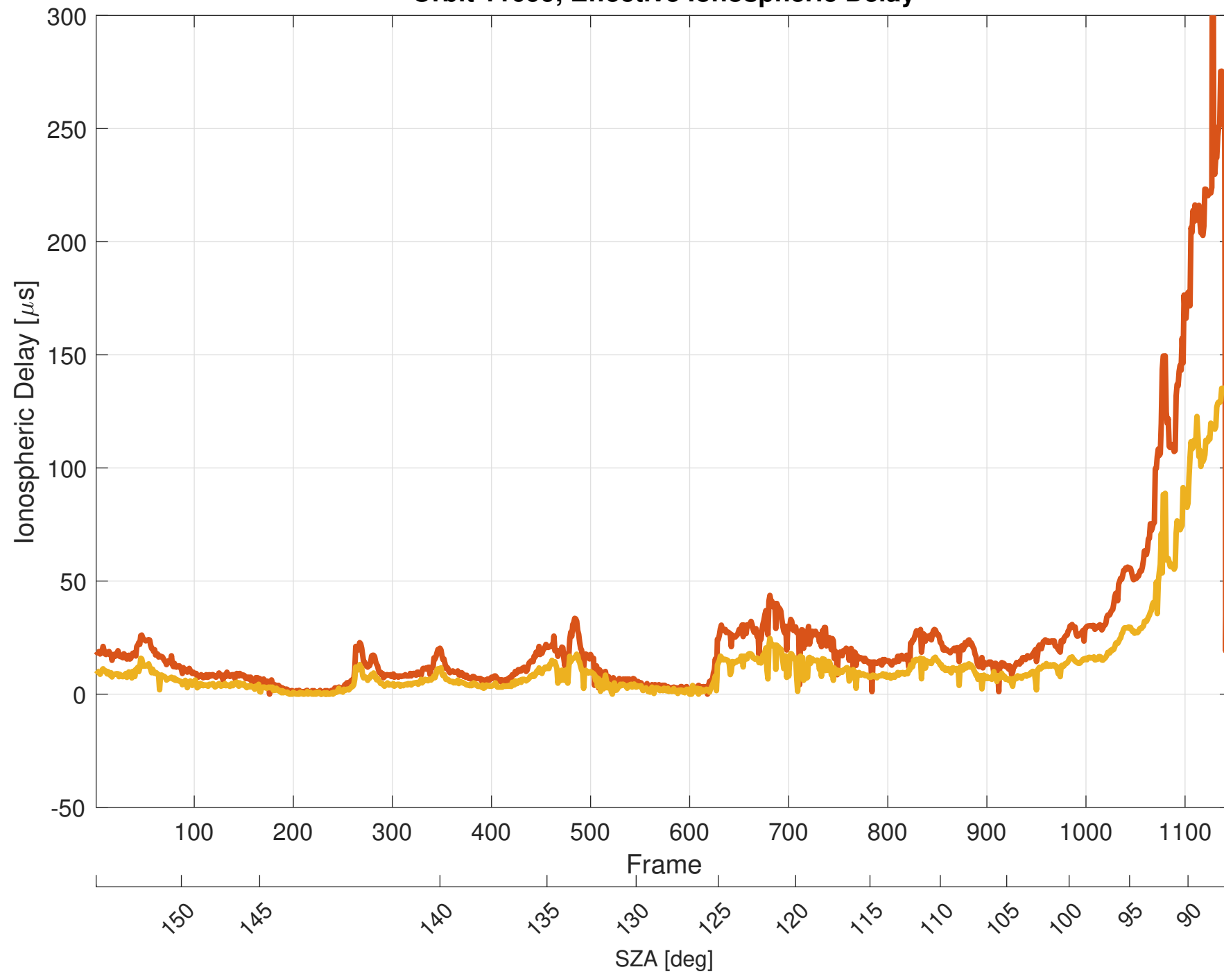
Orbit 11099, Effective Ionospheric Delay
