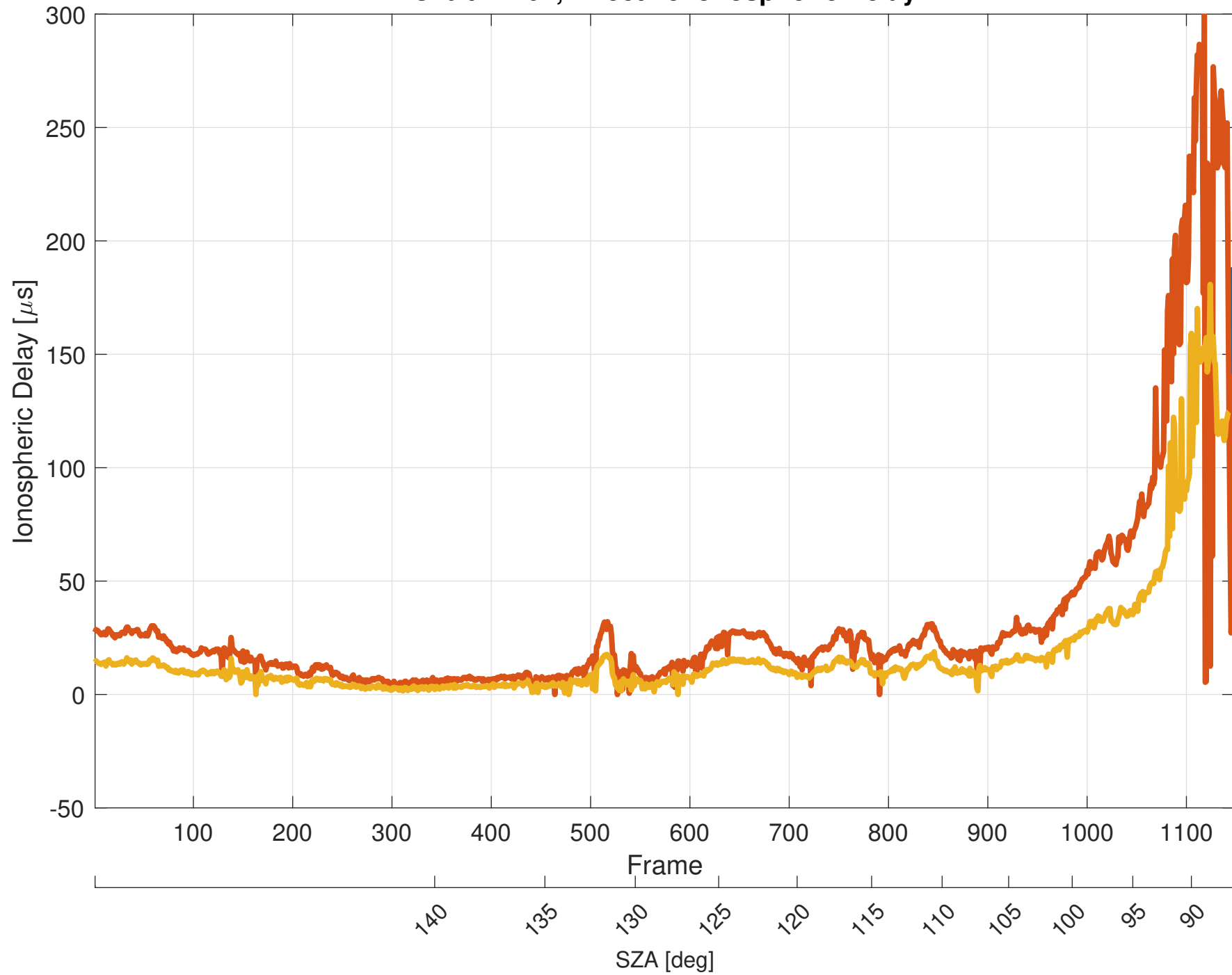
Orbit 11101, Effective Ionospheric Delay
