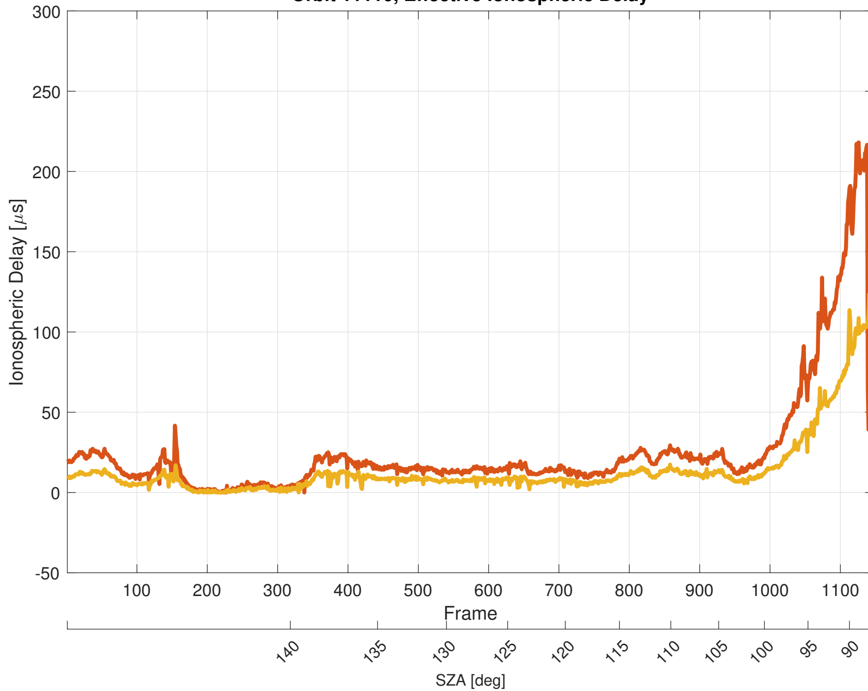
Orbit 11110, Effective Ionospheric Delay
