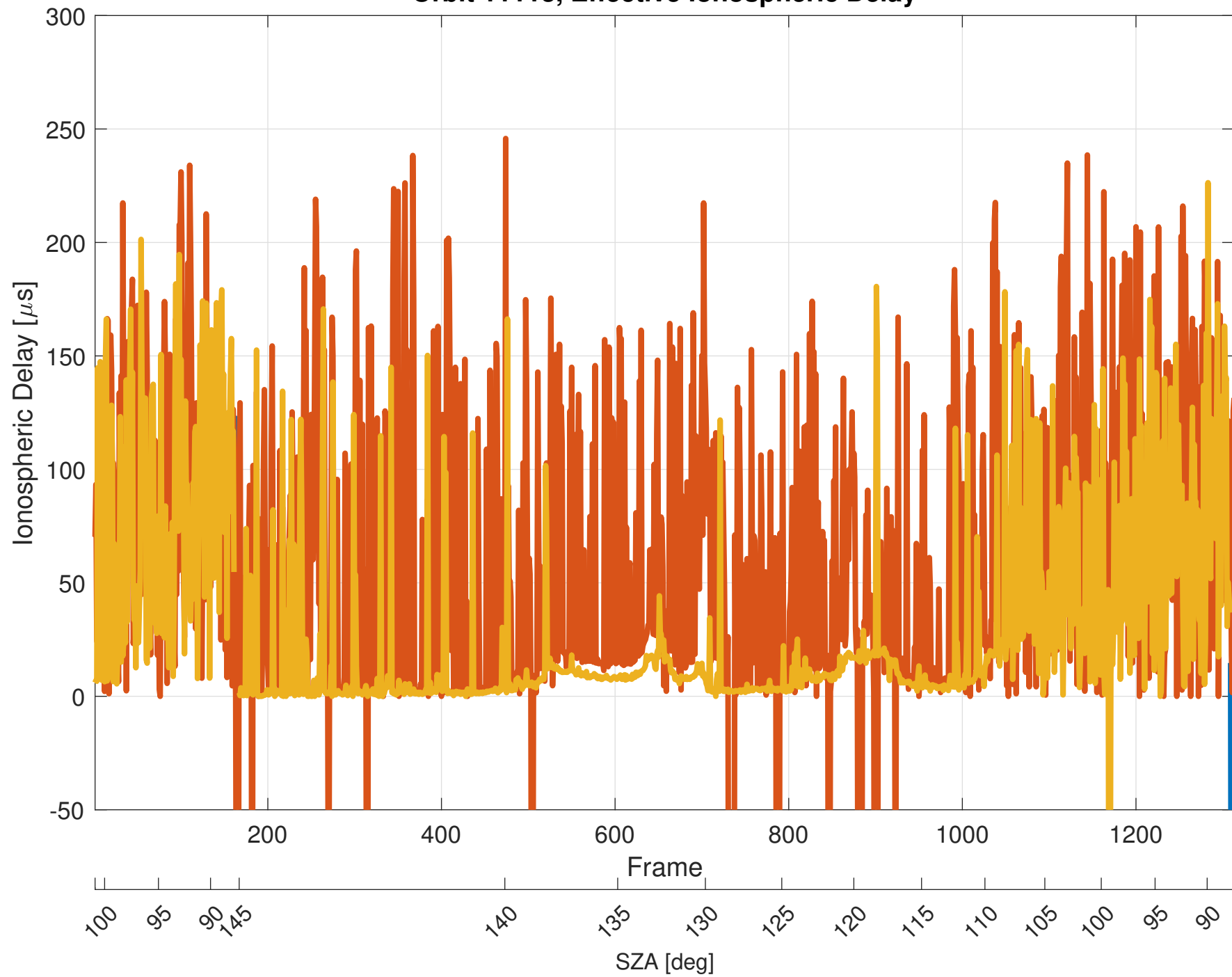
Orbit 11113, Effective Ionospheric Delay
