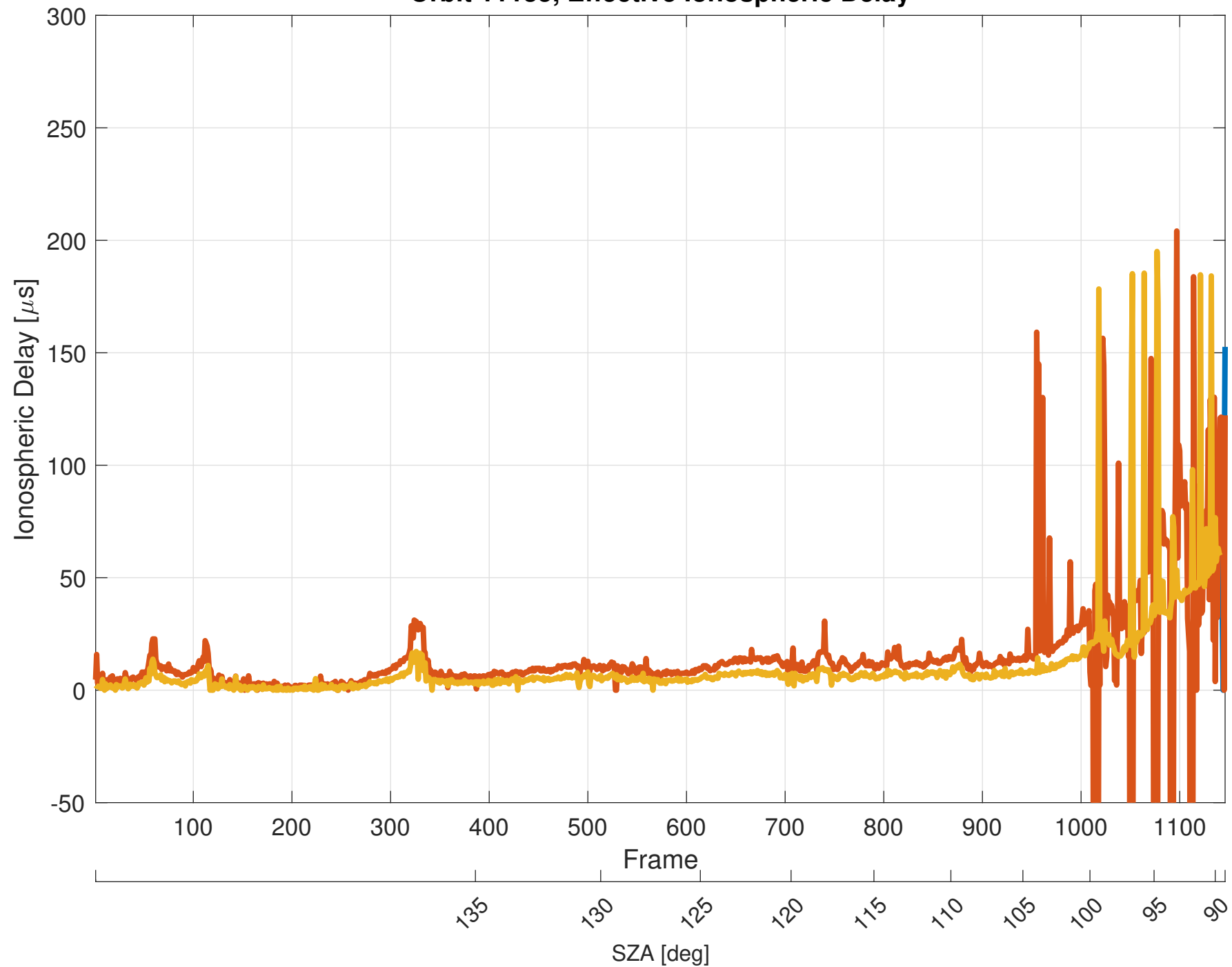
Orbit 11135, Effective Ionospheric Delay
