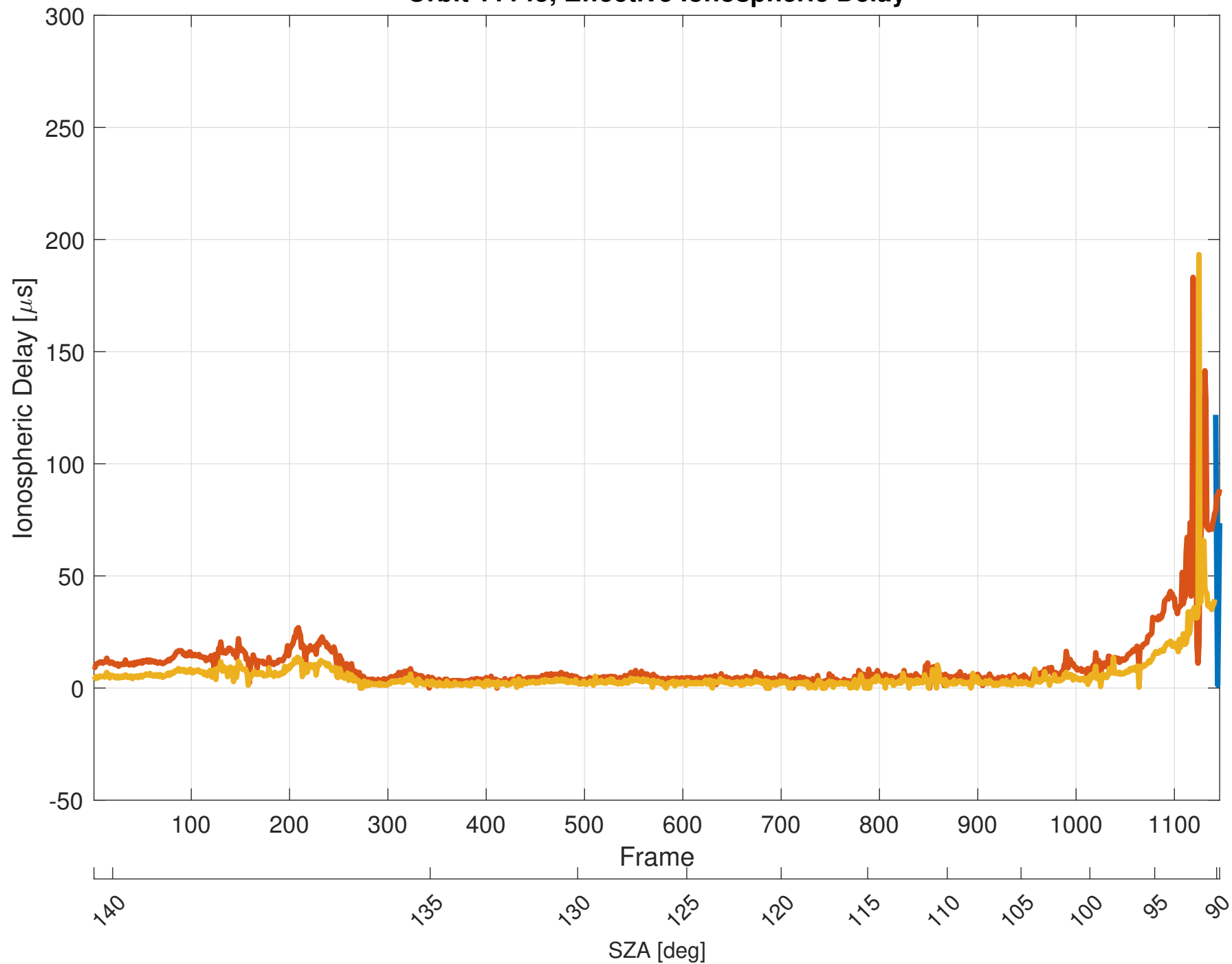
Orbit 11145, Effective Ionospheric Delay
