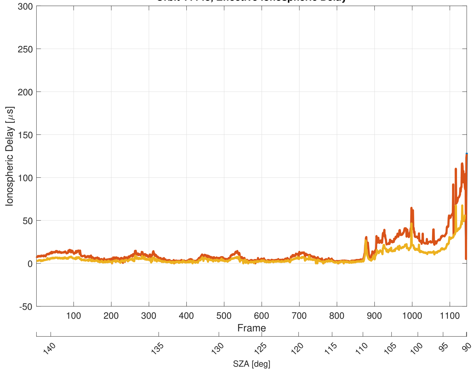
Orbit 11148, Effective Ionospheric Delay
