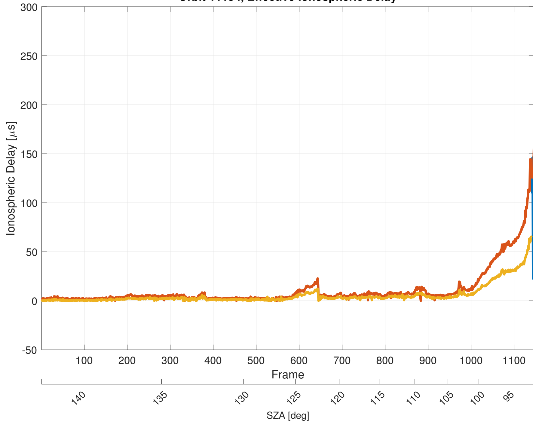
Orbit 11154, Effective Ionospheric Delay
