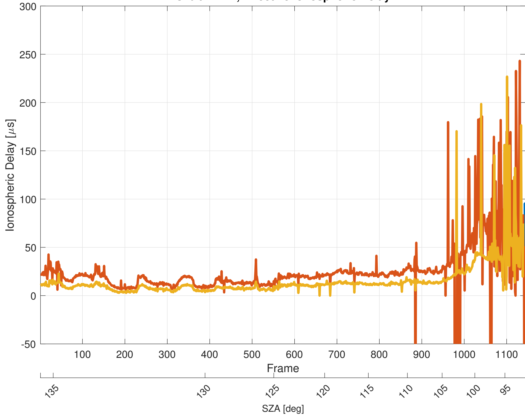
Orbit 11174, Effective Ionospheric Delay
