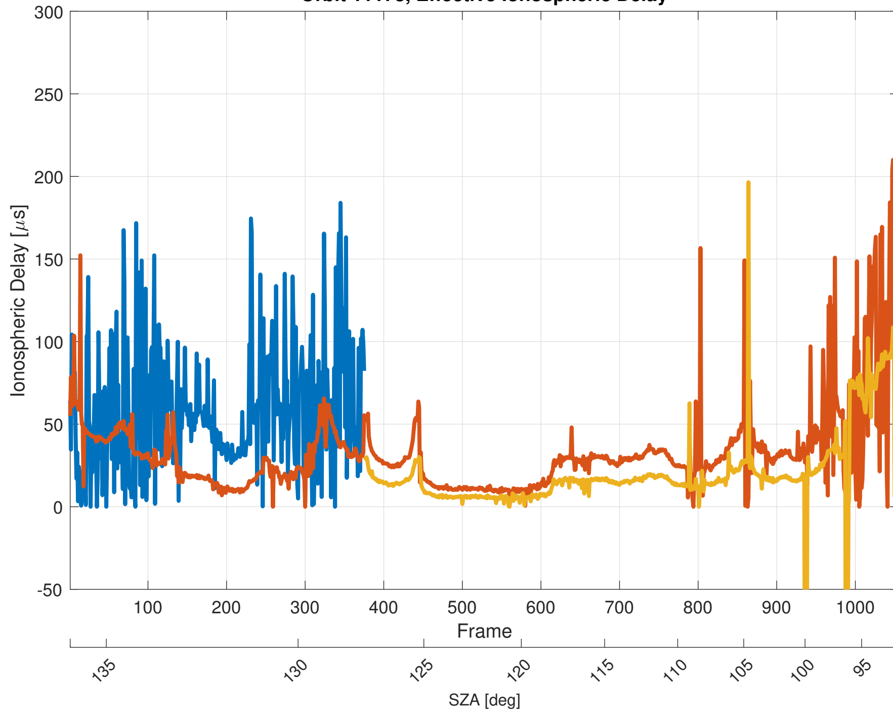
Orbit 11178, Effective Ionospheric Delay
