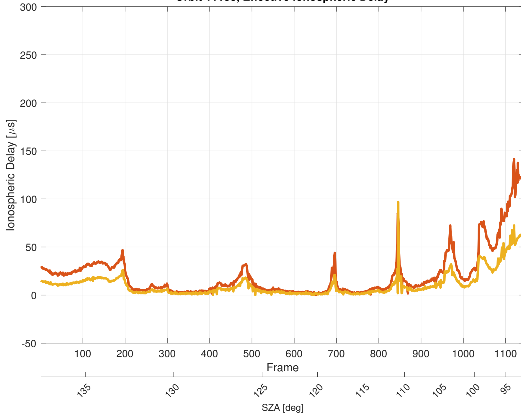
Orbit 11183, Effective Ionospheric Delay
