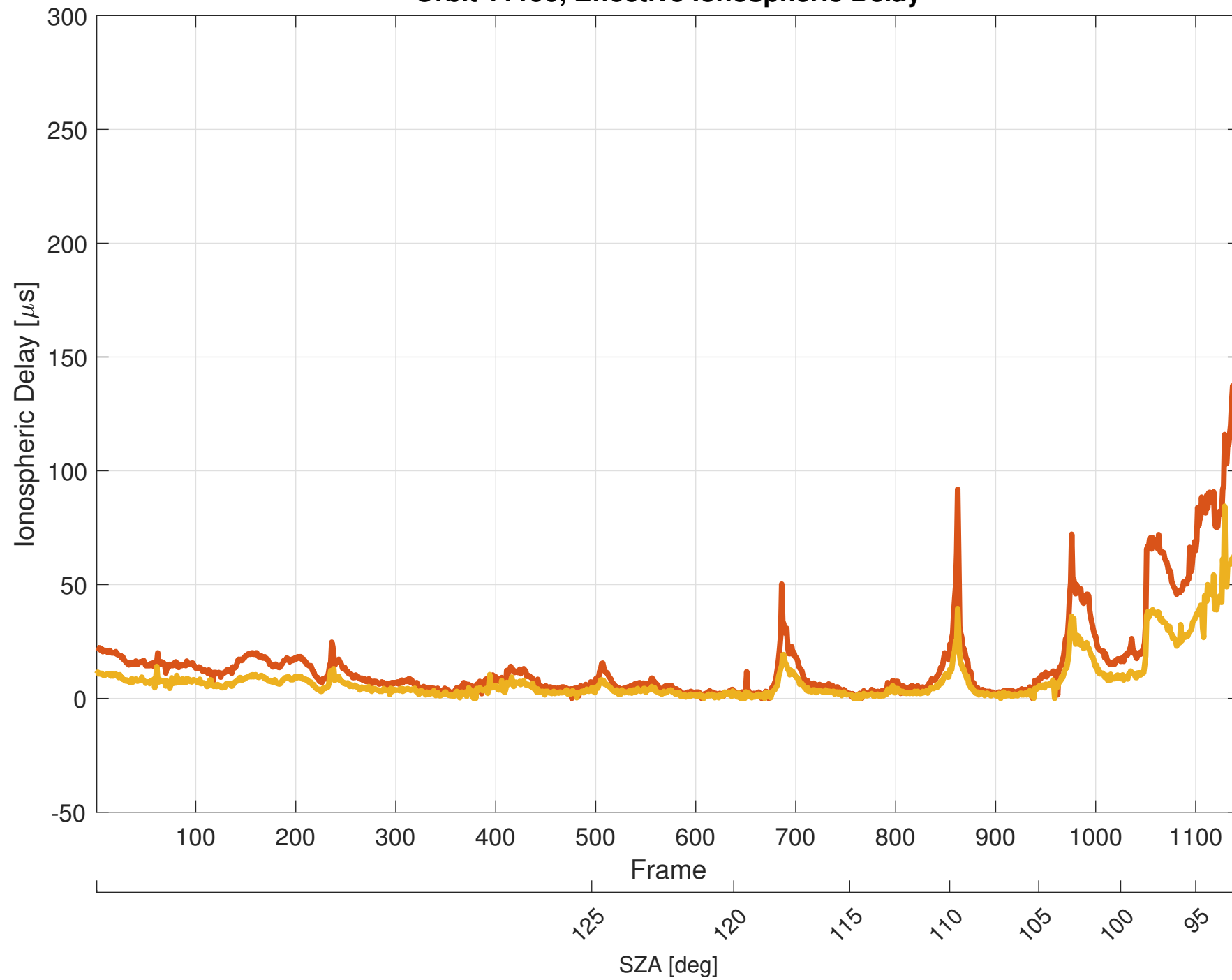
Orbit 11190, Effective Ionospheric Delay
