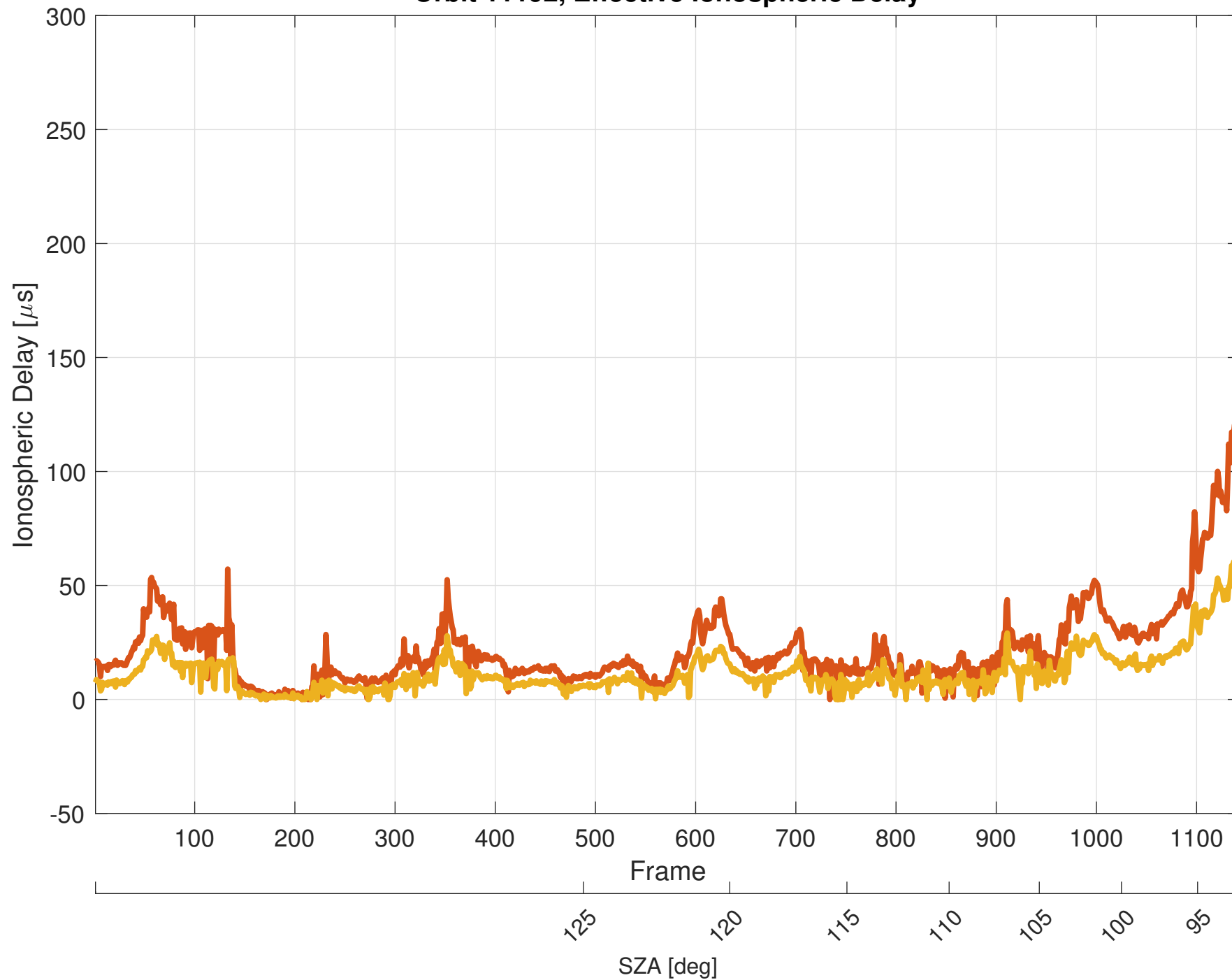
Orbit 11192, Effective Ionospheric Delay
