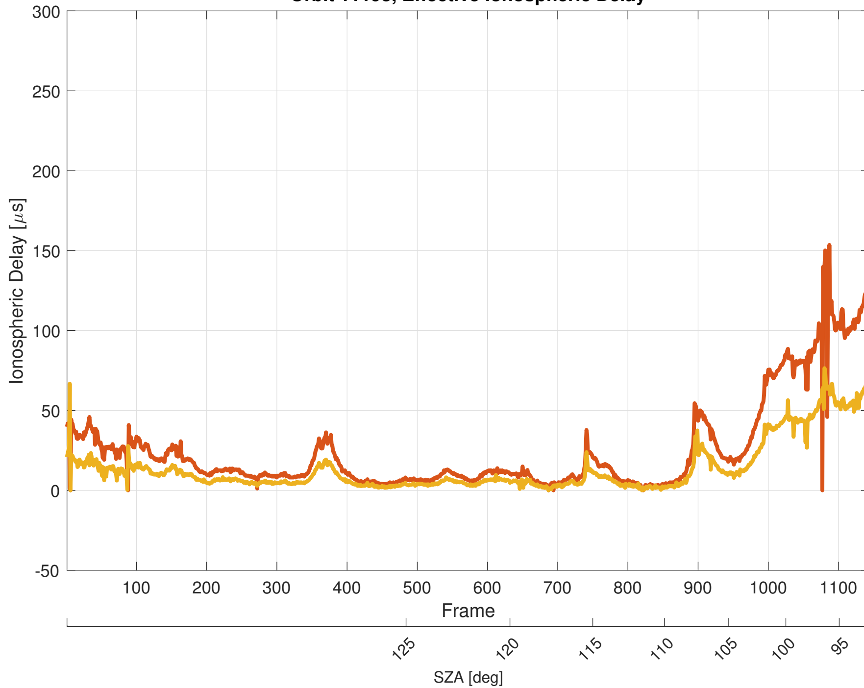
Orbit 11193, Effective Ionospheric Delay
