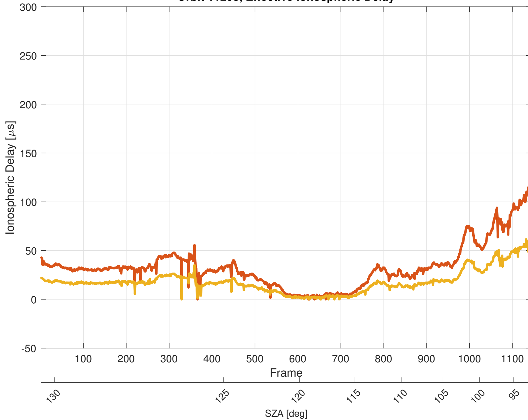
Orbit 11203, Effective Ionospheric Delay
