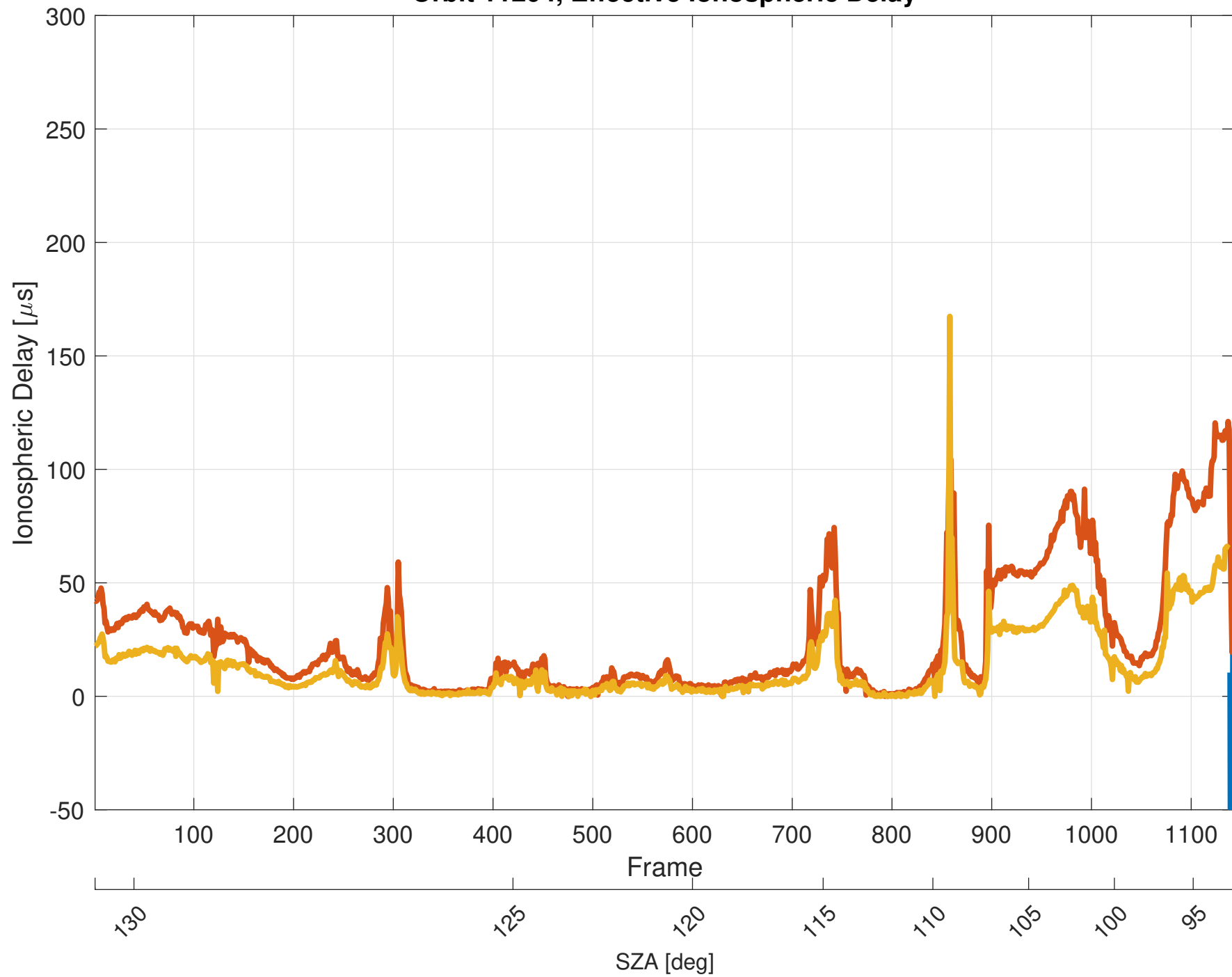
Orbit 11204, Effective Ionospheric Delay
