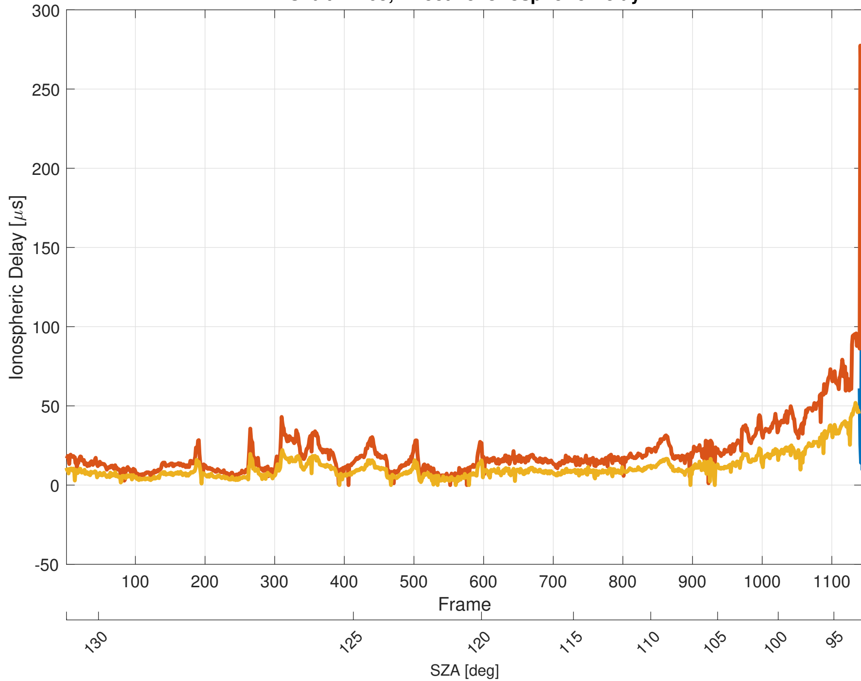
Orbit 11205, Effective Ionospheric Delay
