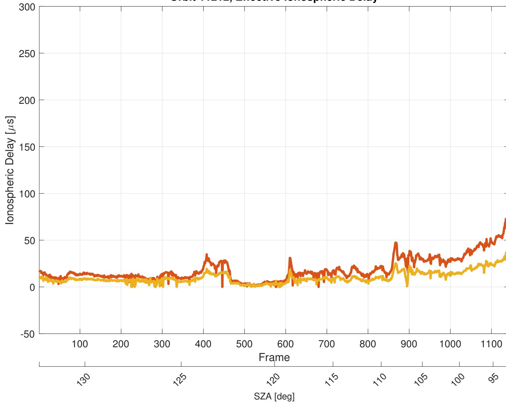
Orbit 11212, Effective Ionospheric Delay
