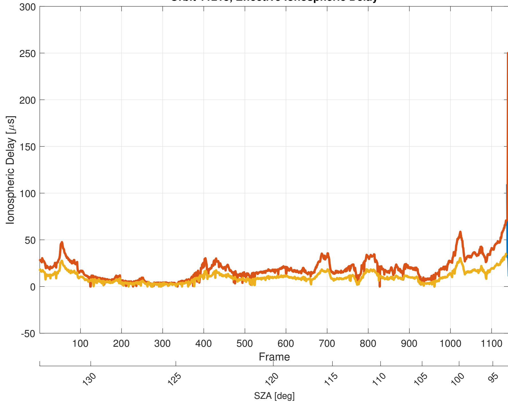
Orbit 11213, Effective Ionospheric Delay
