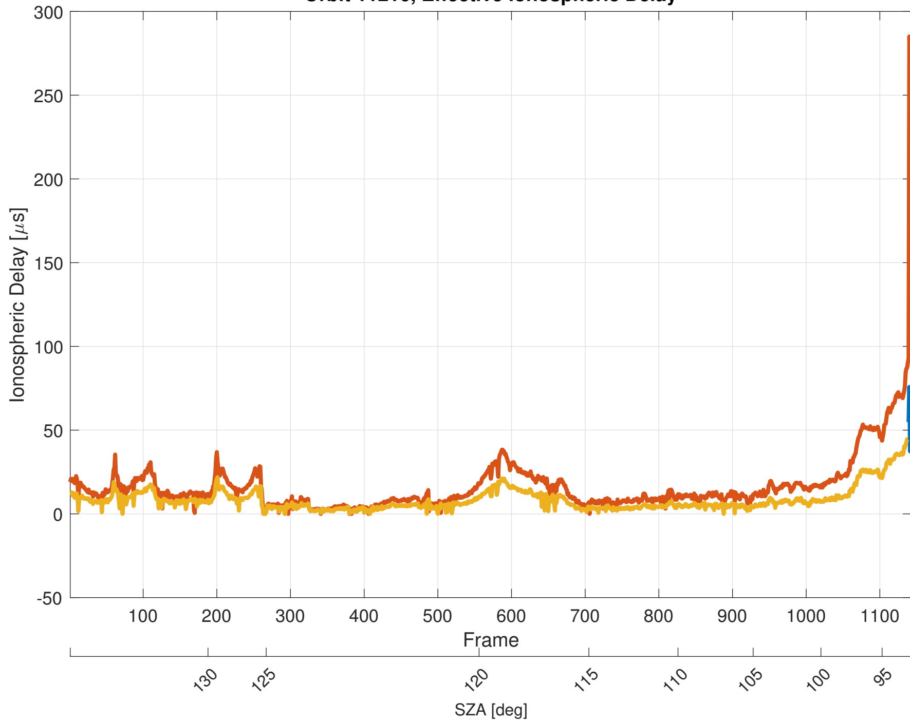
Orbit 11216, Effective Ionospheric Delay
