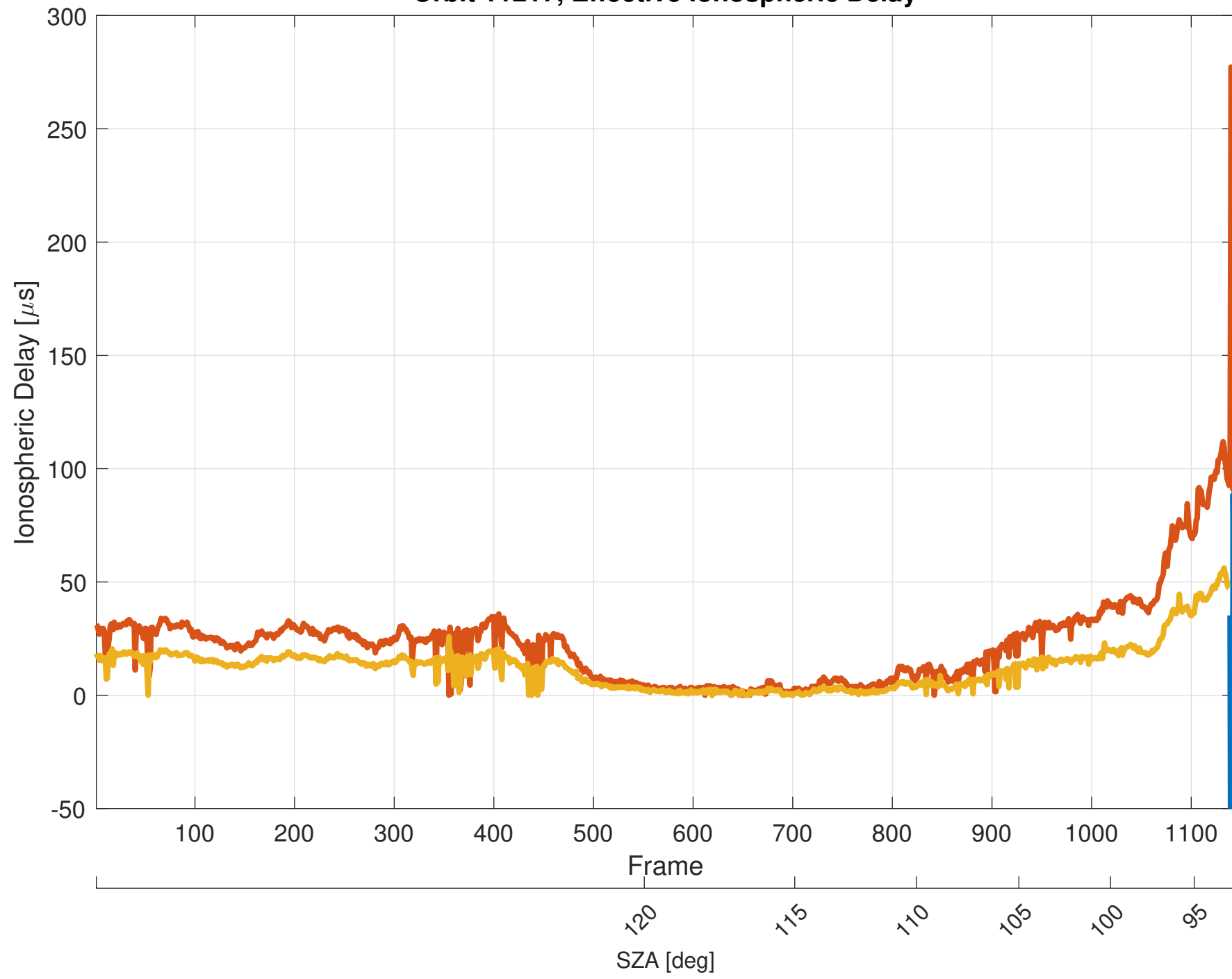
Orbit 11217, Effective Ionospheric Delay
