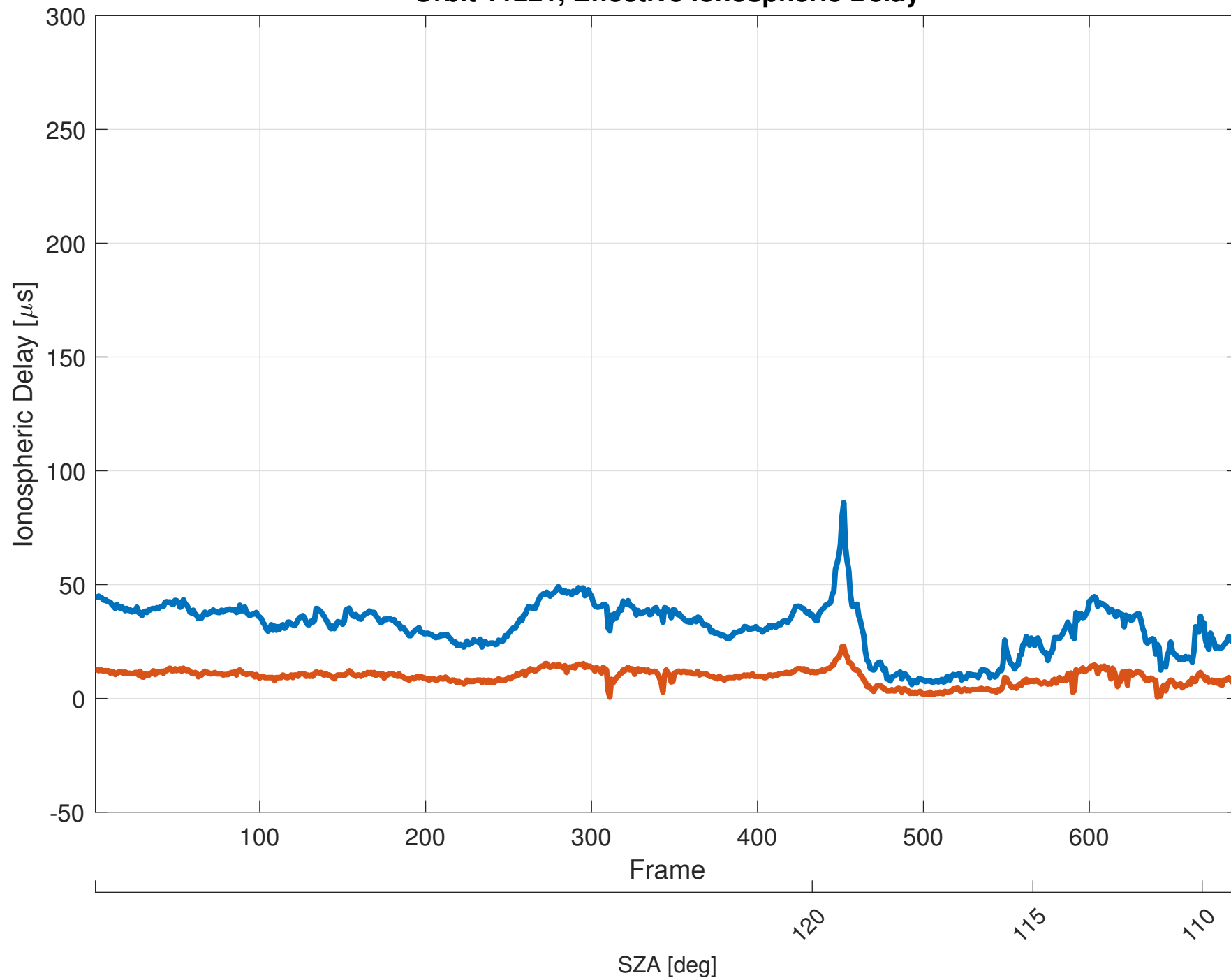
Orbit 11221, Effective Ionospheric Delay
