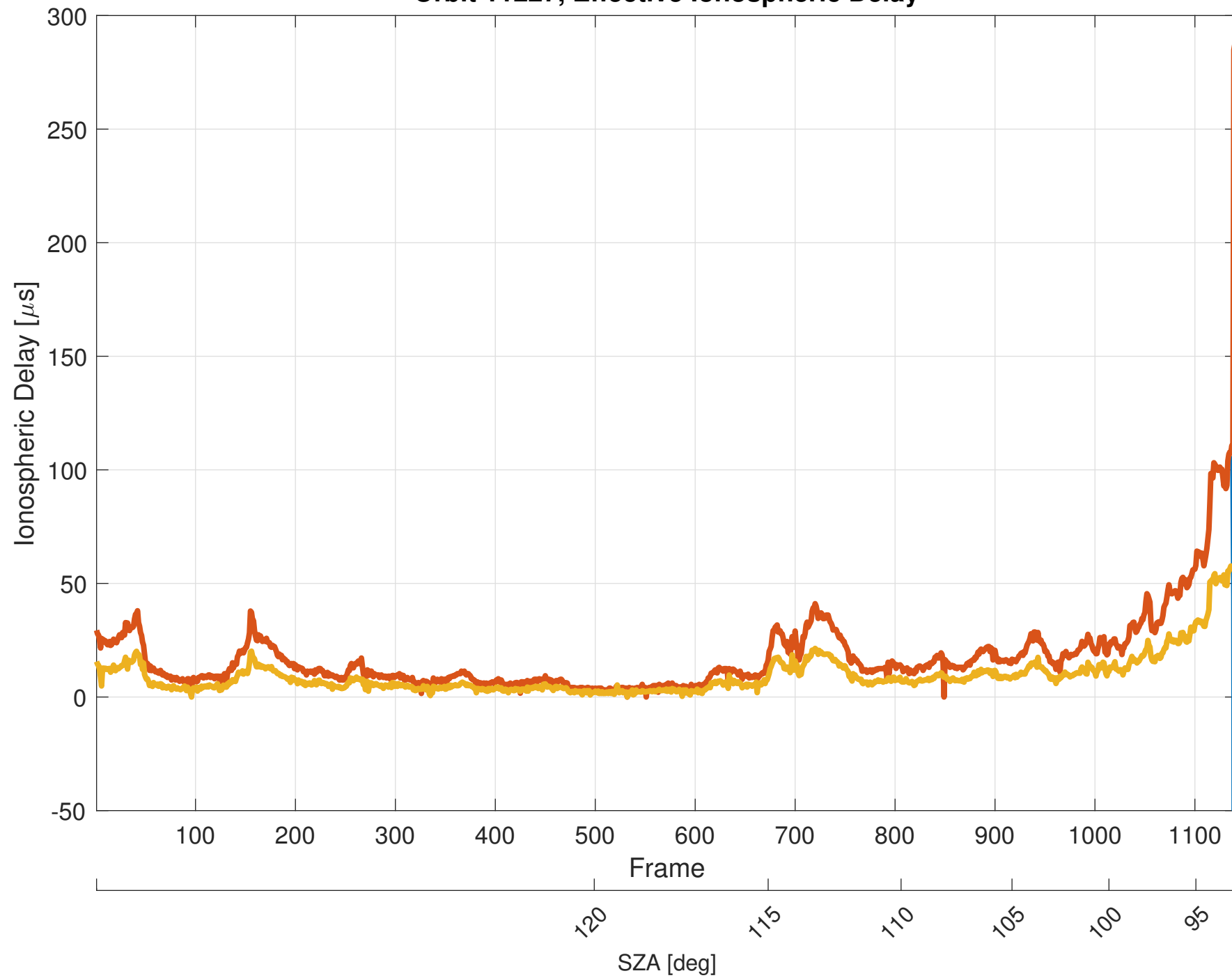
Orbit 11227, Effective Ionospheric Delay
