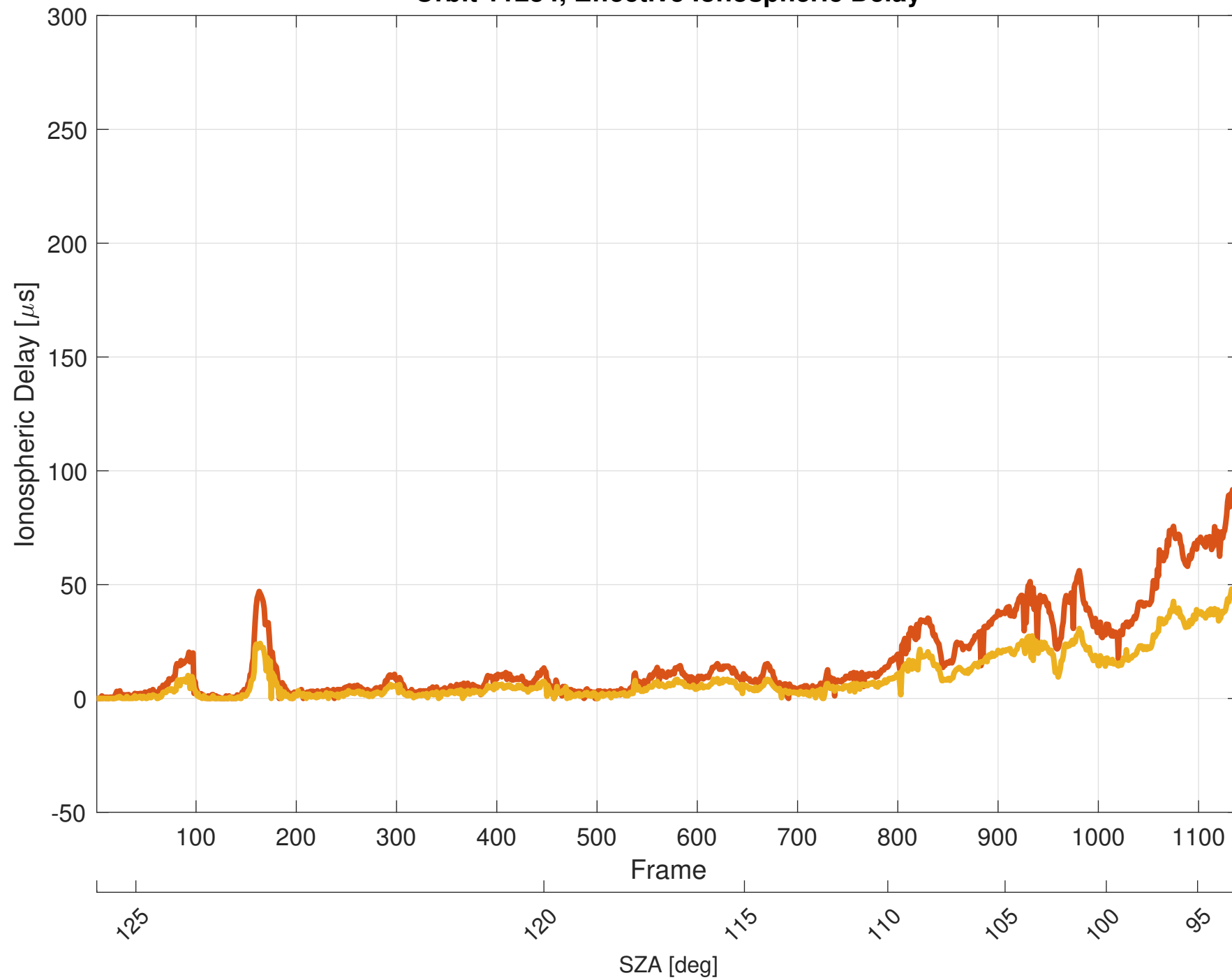
Orbit 11234, Effective Ionospheric Delay
