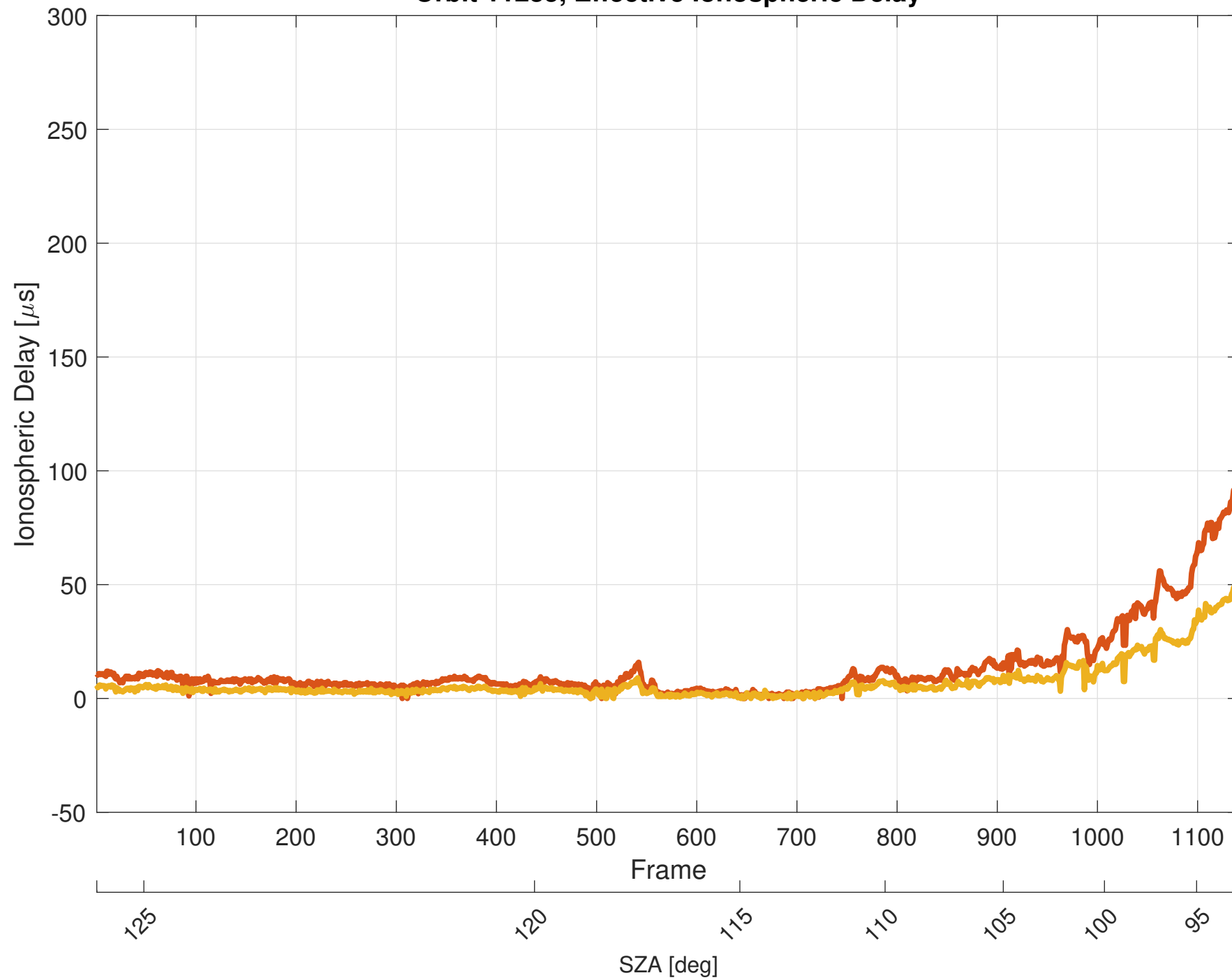
Orbit 11235, Effective Ionospheric Delay
