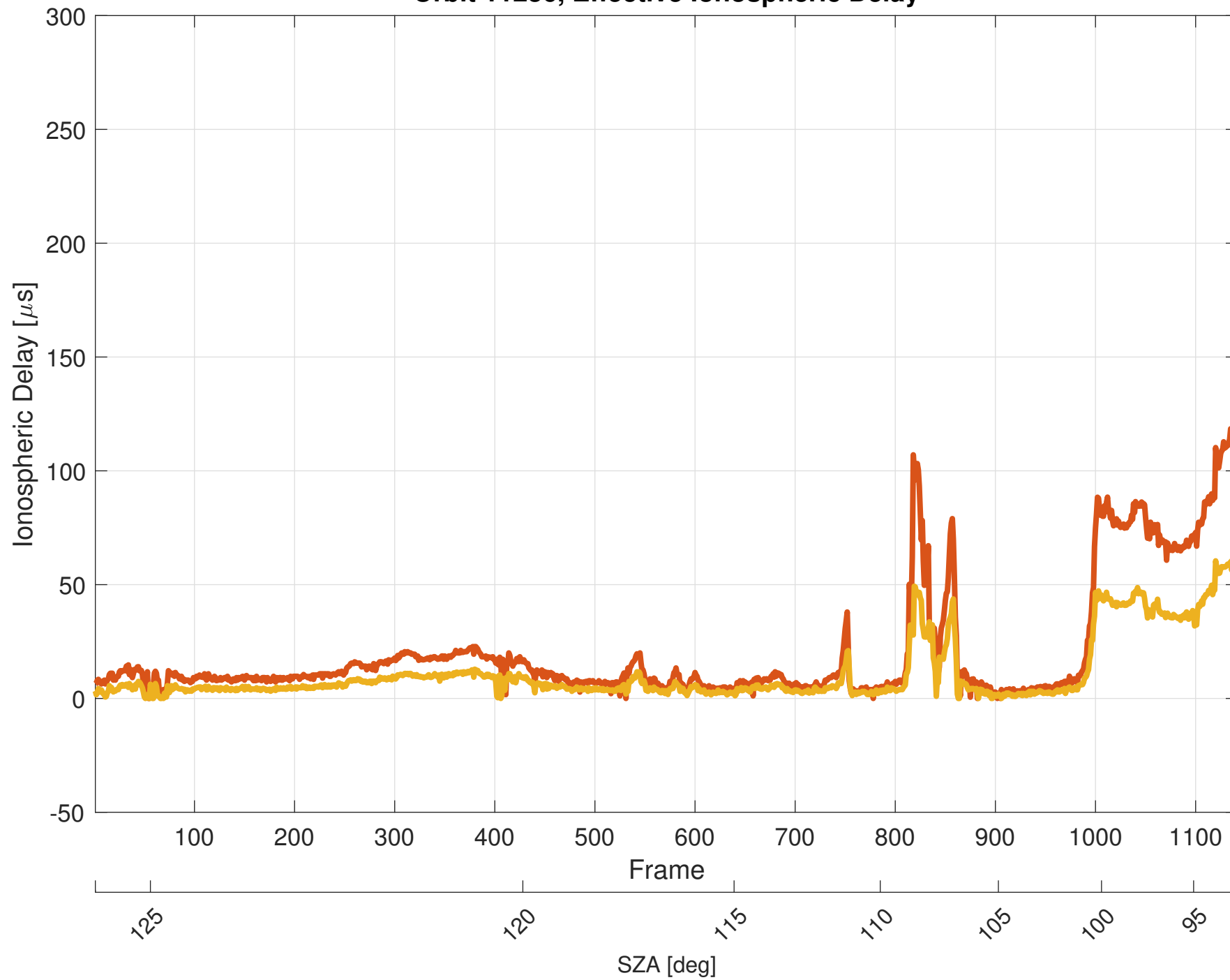
Orbit 11236, Effective Ionospheric Delay
