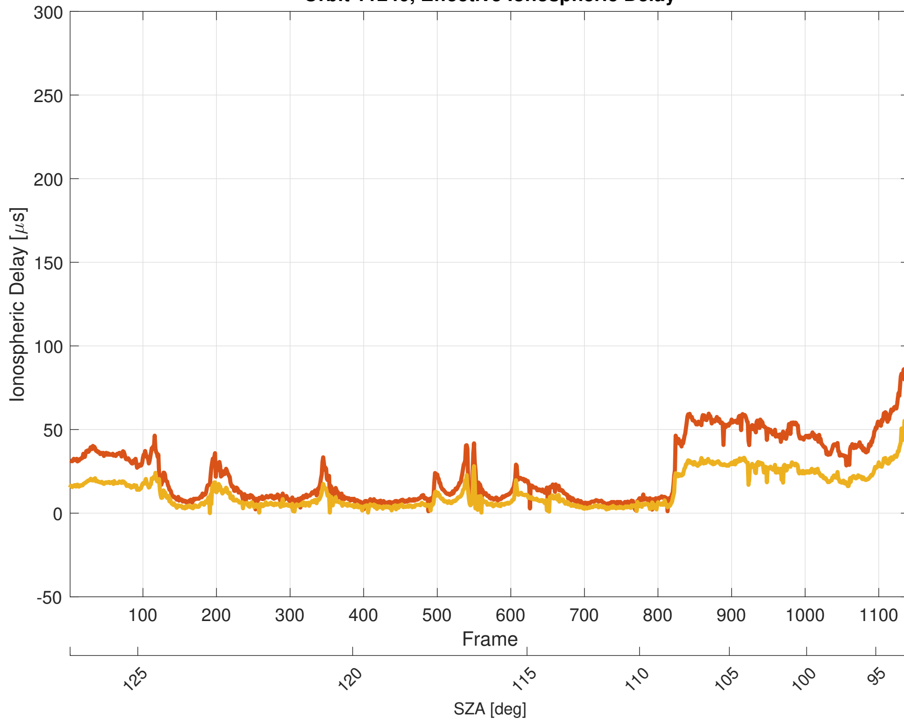
Orbit 11240, Effective Ionospheric Delay
