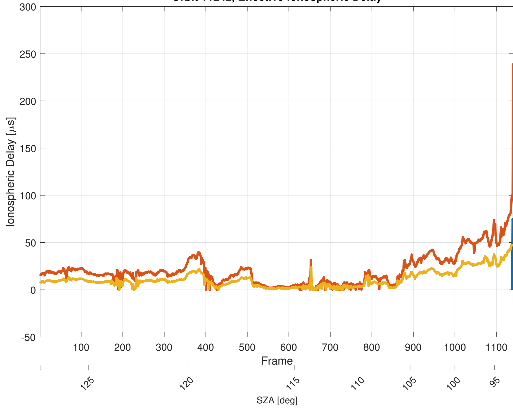
Orbit 11242, Effective Ionospheric Delay
