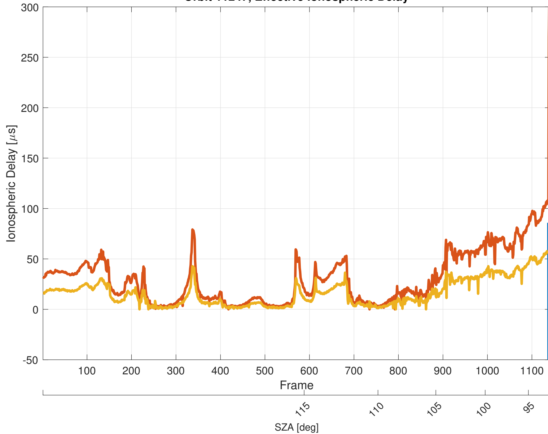
Orbit 11247, Effective Ionospheric Delay
