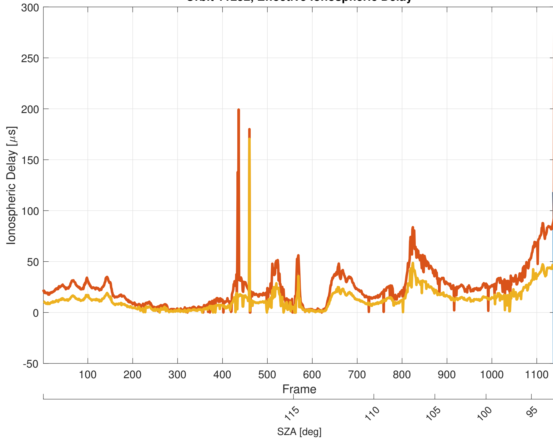
Orbit 11252, Effective Ionospheric Delay
