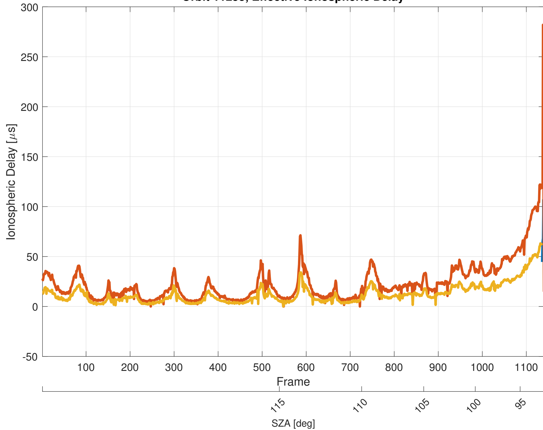
Orbit 11255, Effective Ionospheric Delay
