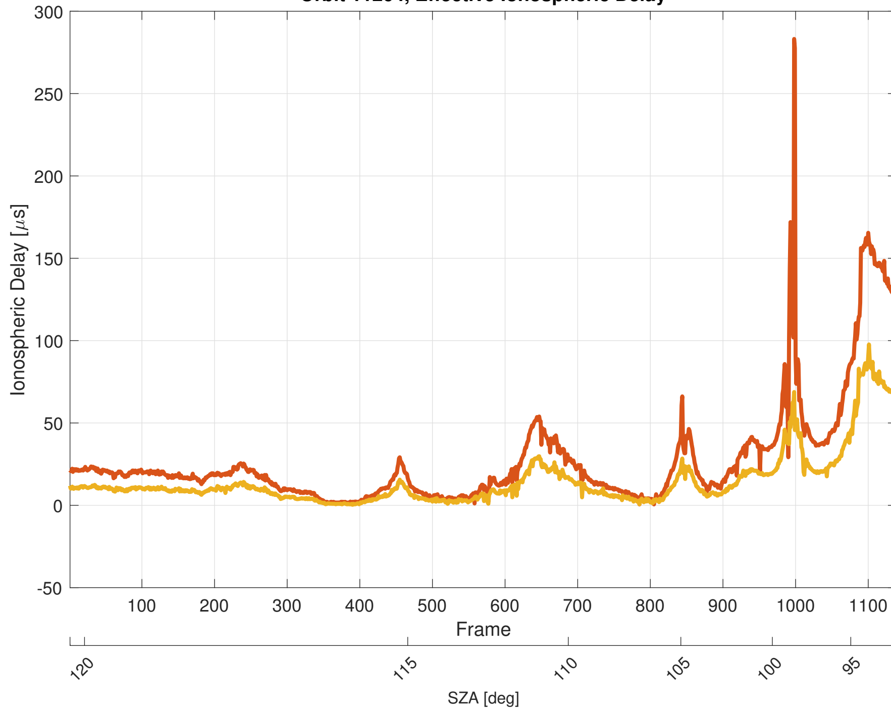
Orbit 11264, Effective Ionospheric Delay
