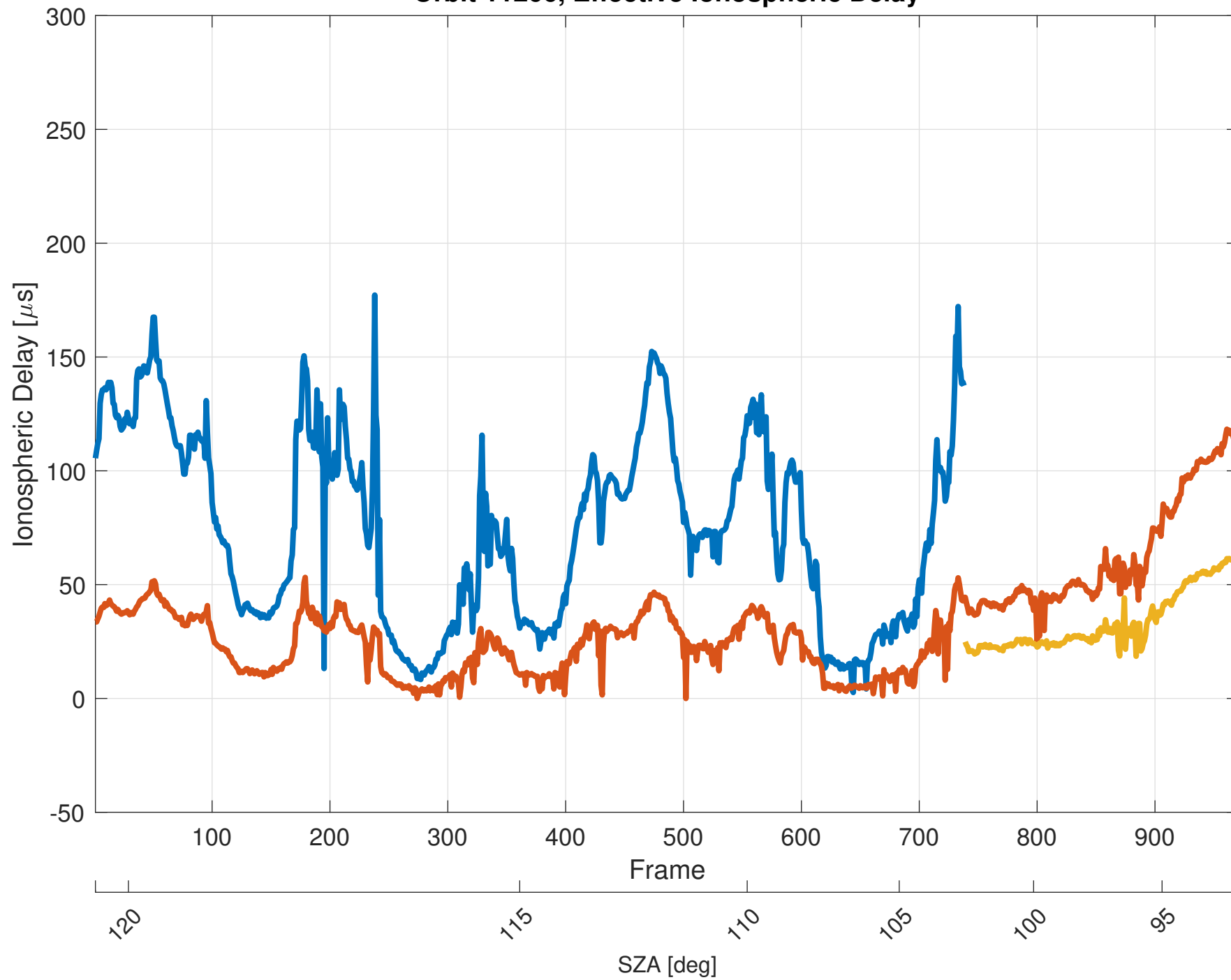
Orbit 11266, Effective Ionospheric Delay
