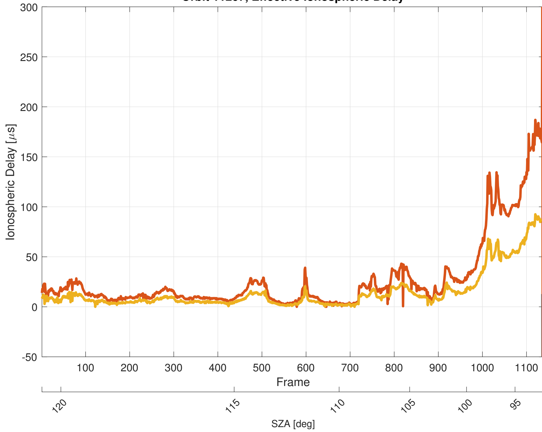
Orbit 11267, Effective Ionospheric Delay
