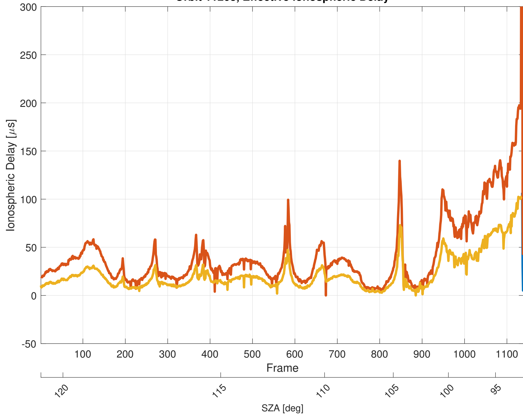
Orbit 11268, Effective Ionospheric Delay
