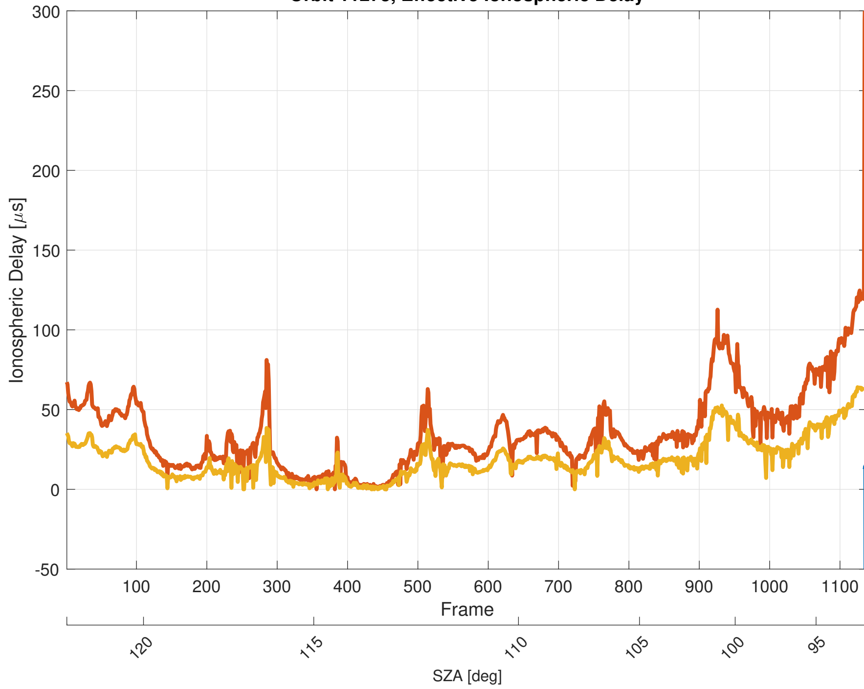
Orbit 11273, Effective Ionospheric Delay
