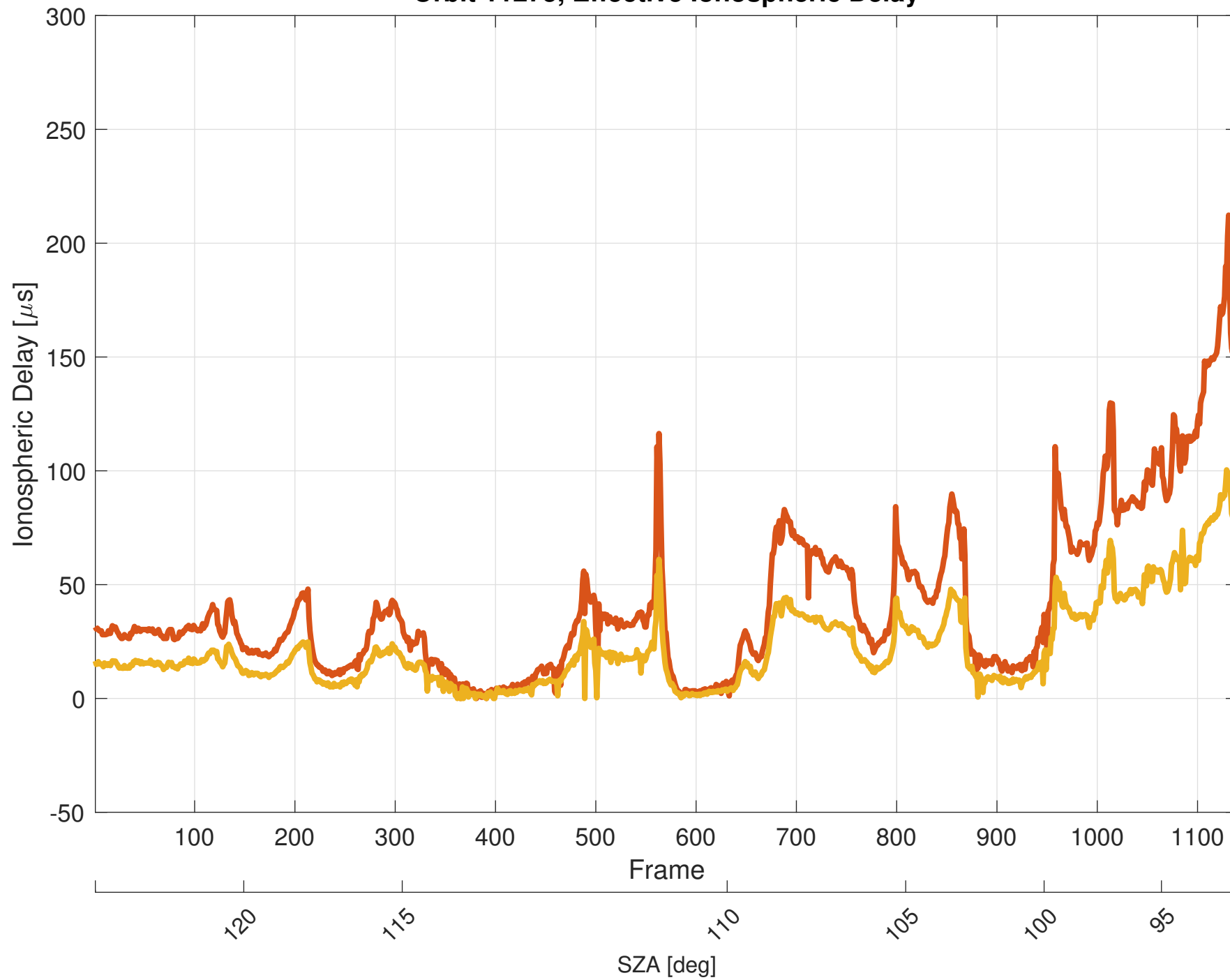
Orbit 11275, Effective Ionospheric Delay
