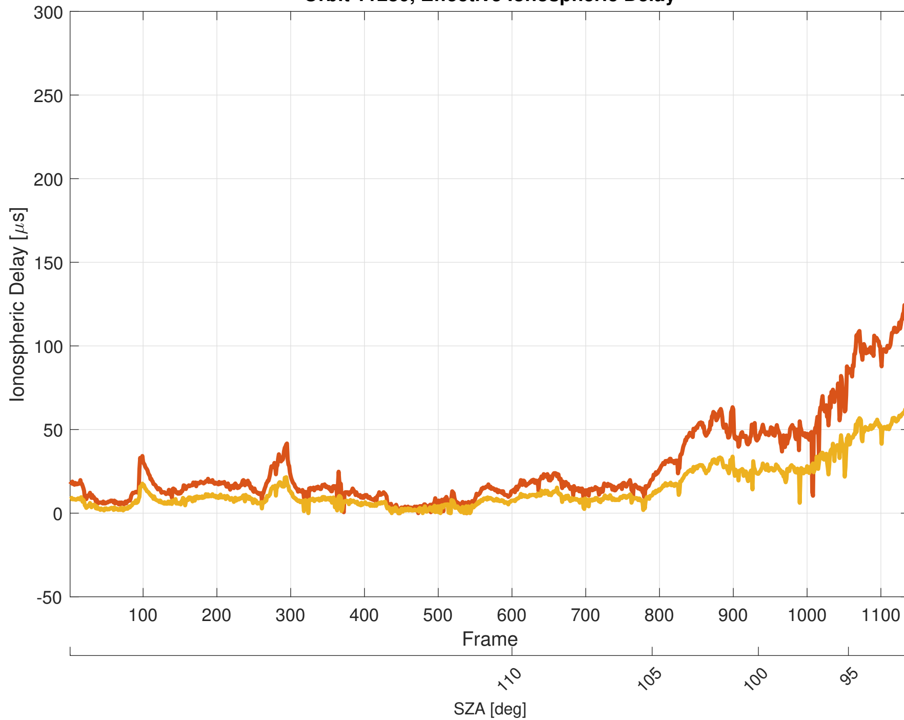
Orbit 11280, Effective Ionospheric Delay
