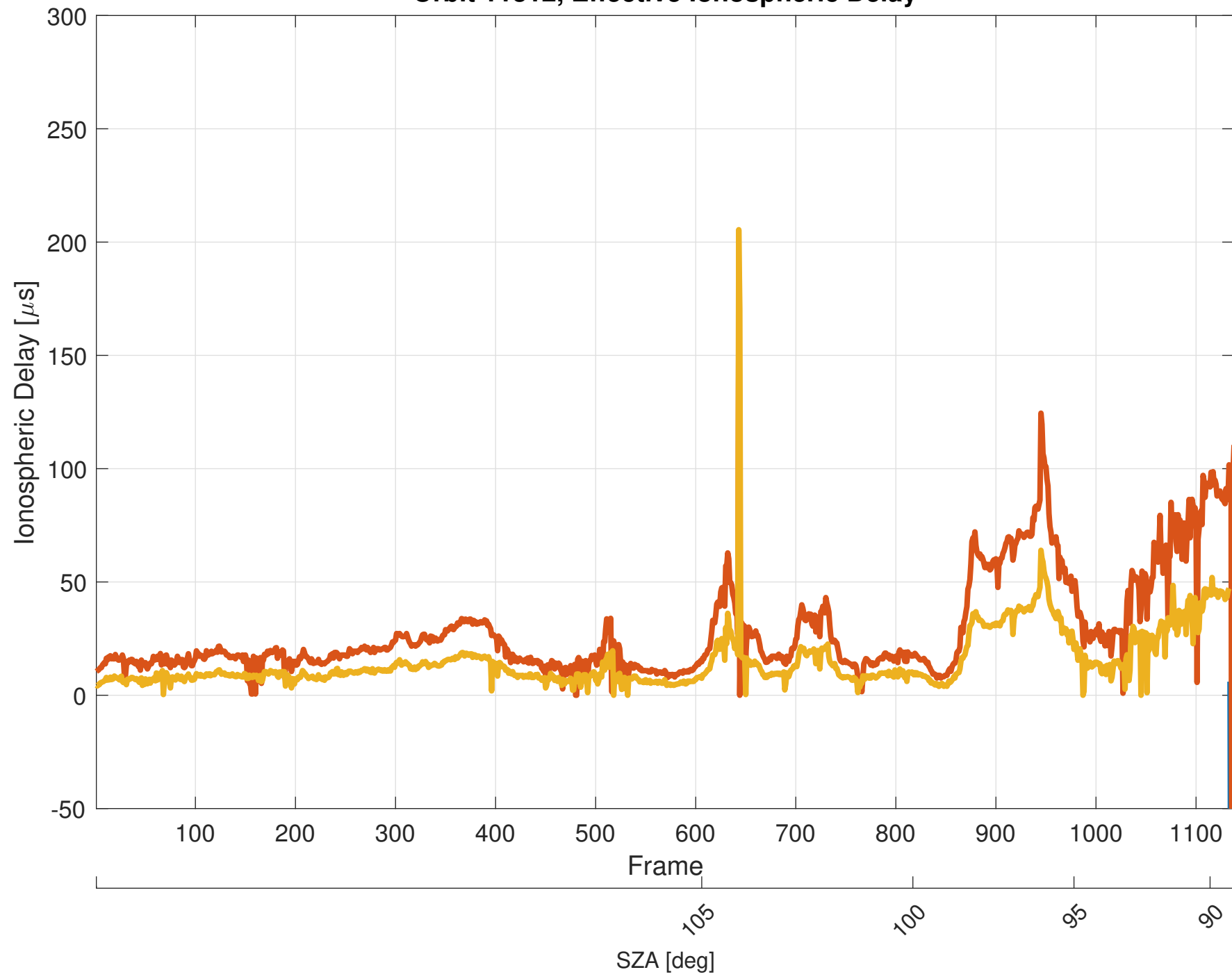
Orbit 11312, Effective Ionospheric Delay
