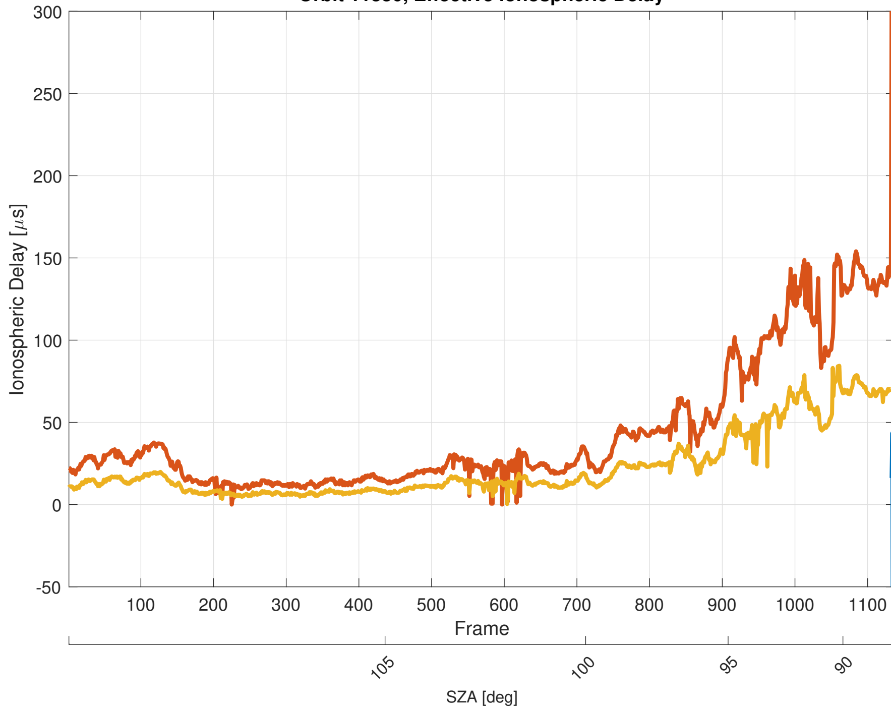
Orbit 11330, Effective Ionospheric Delay
