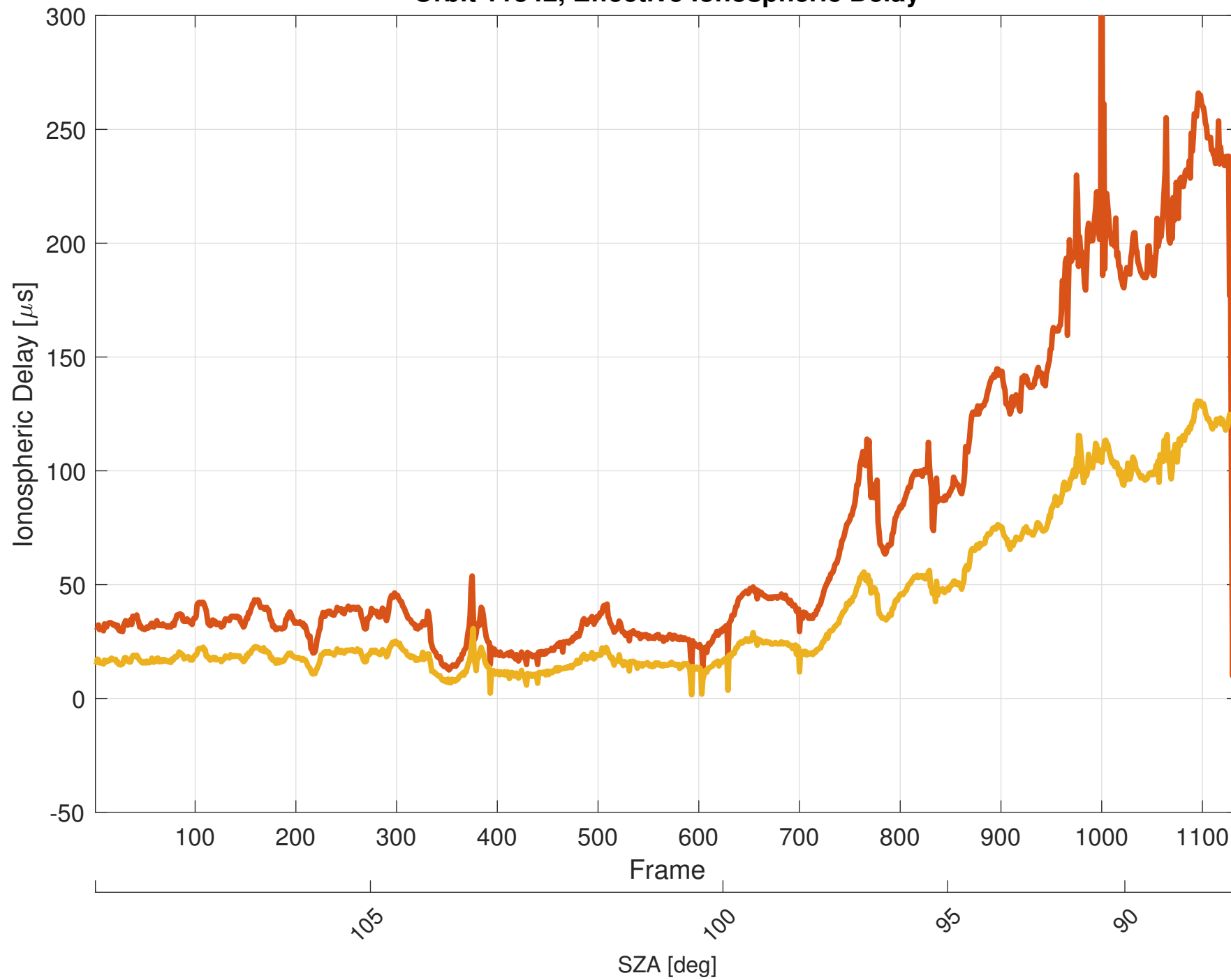
Orbit 11342, Effective Ionospheric Delay
