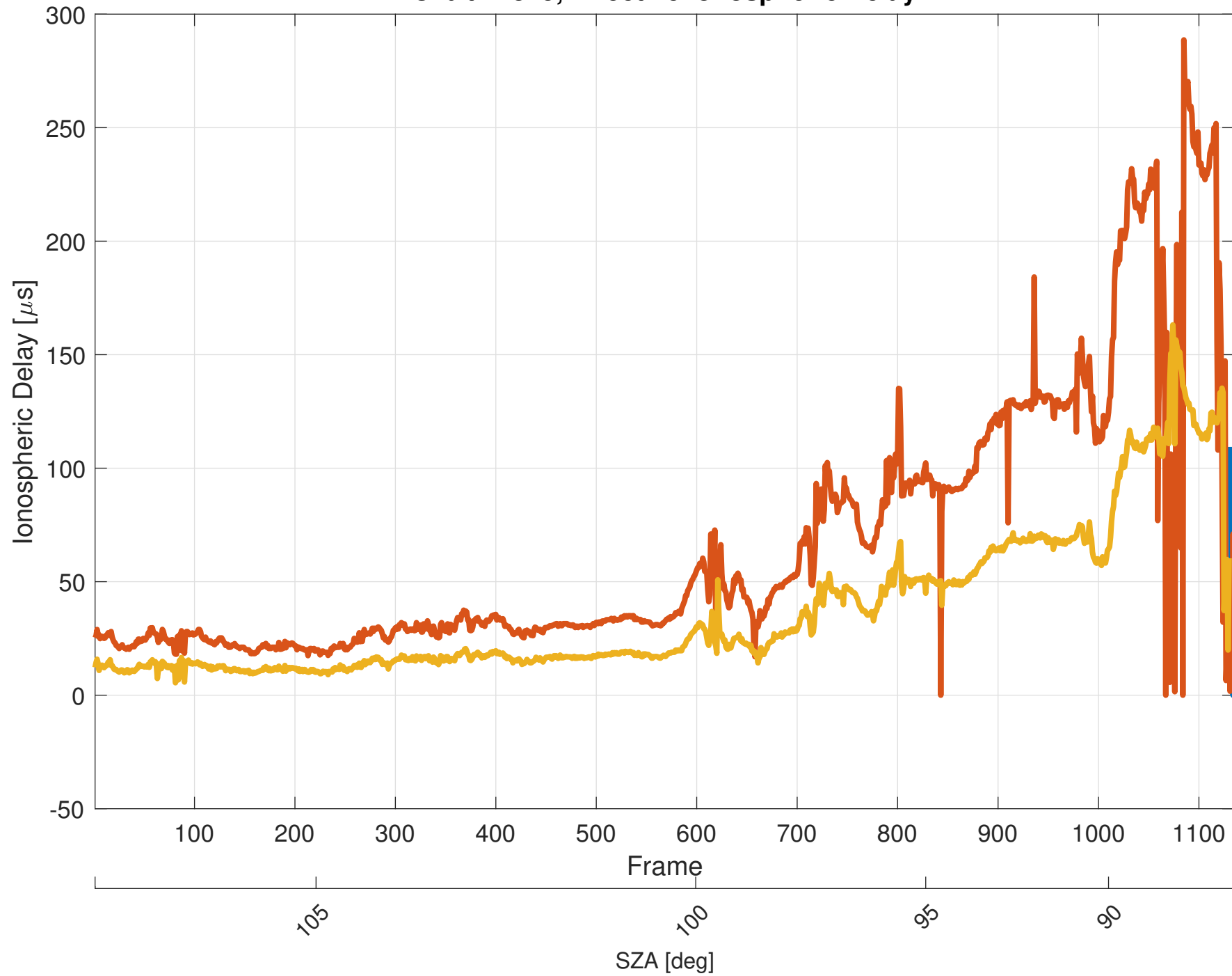
Orbit 11345, Effective Ionospheric Delay
