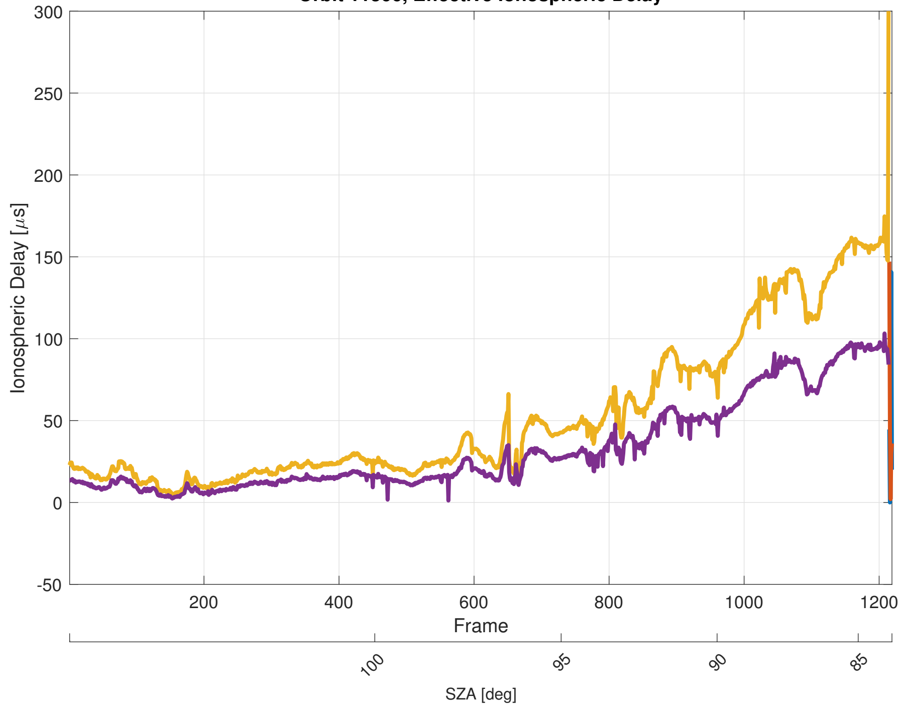
Orbit 11366, Effective Ionospheric Delay
