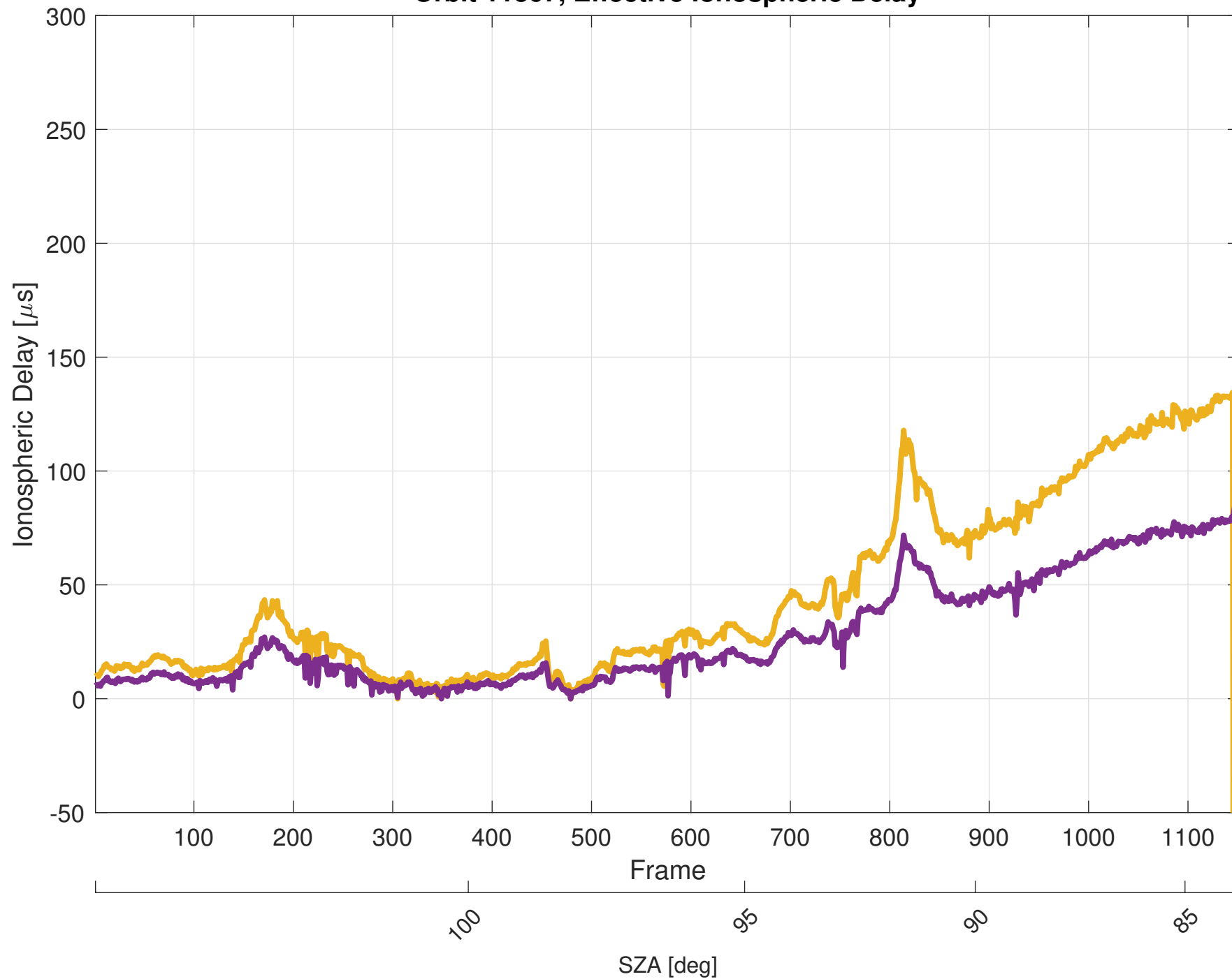
Orbit 11367, Effective Ionospheric Delay
