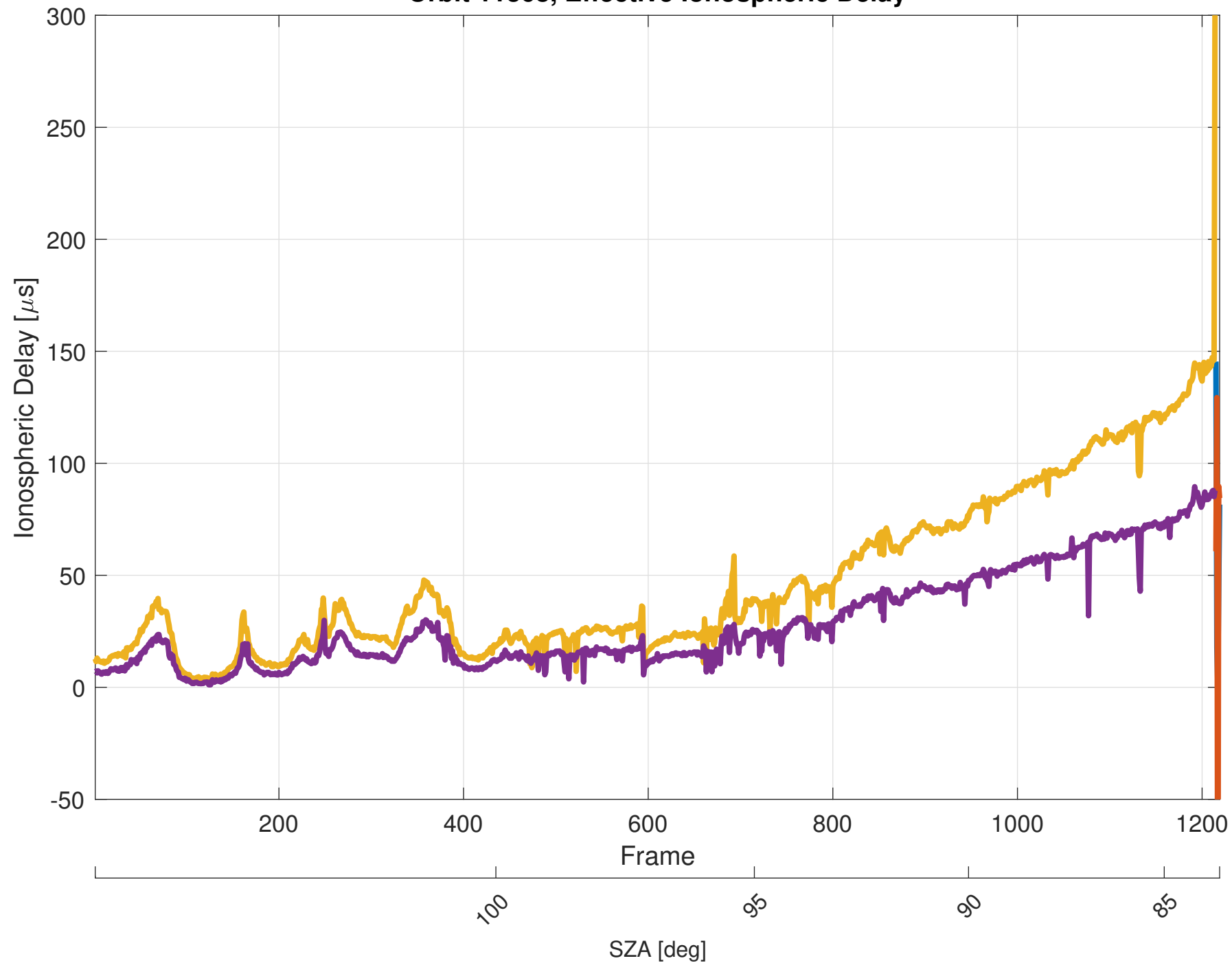
Orbit 11368, Effective Ionospheric Delay
