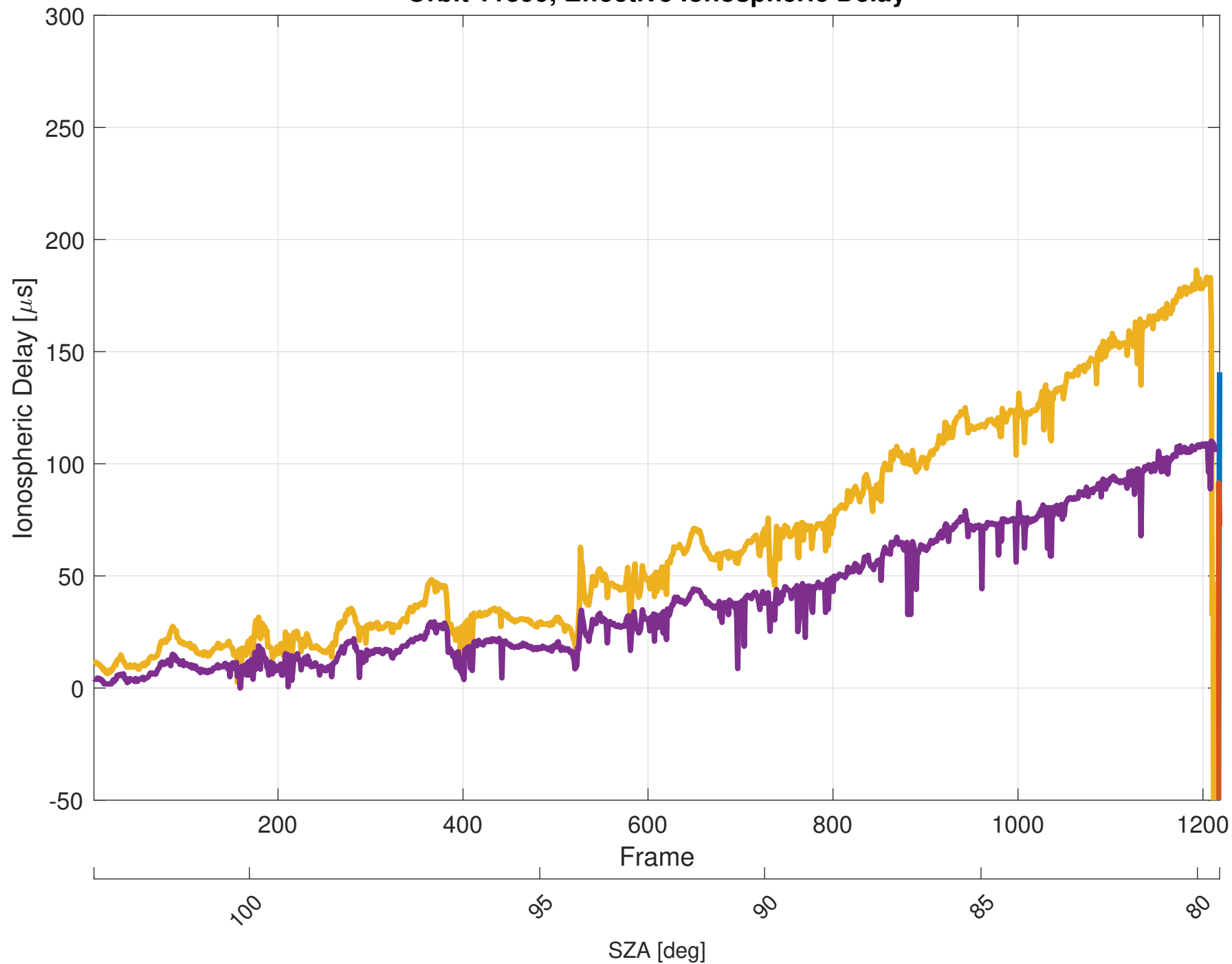
Orbit 11399, Effective Ionospheric Delay
