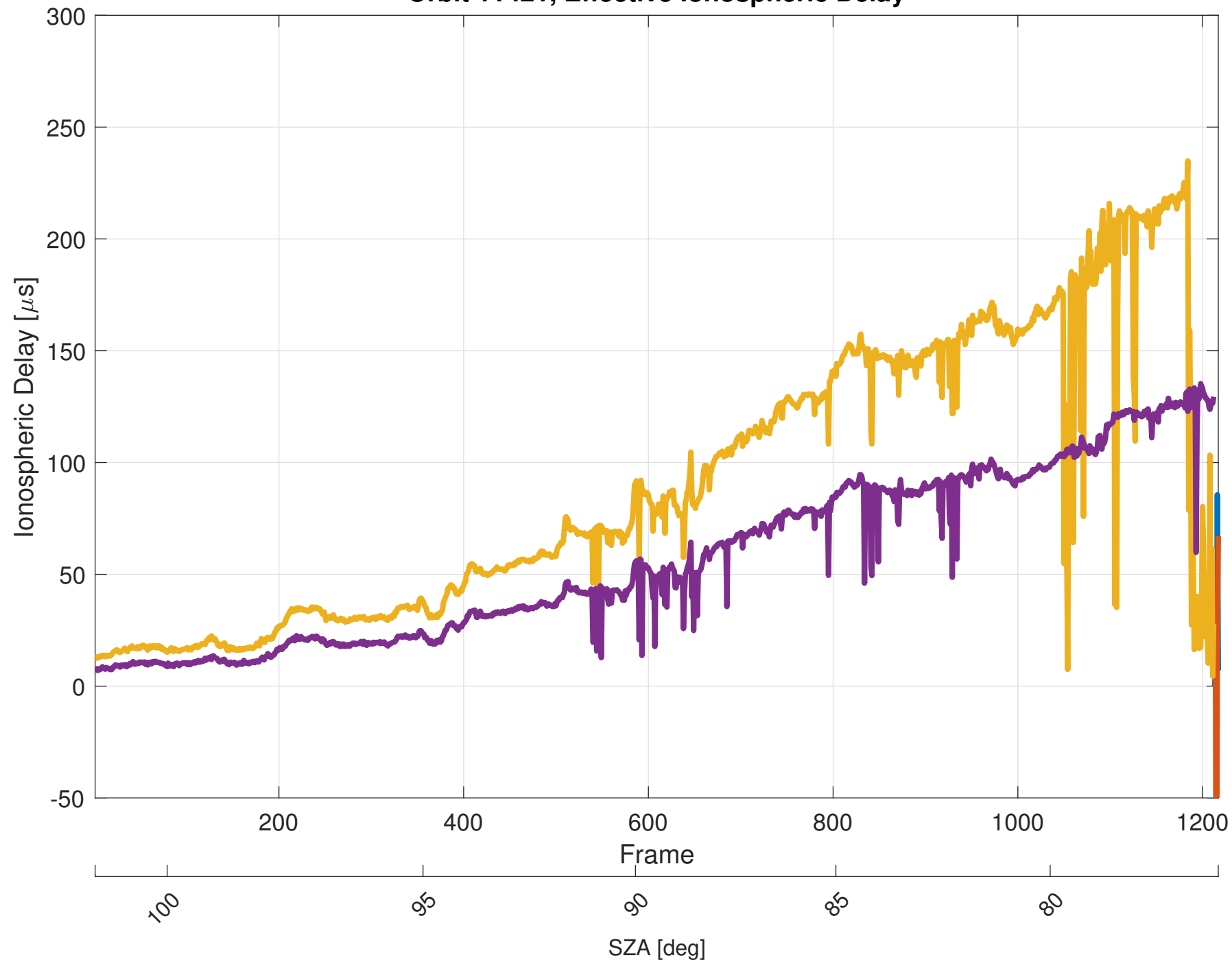
Orbit 11421, Effective Ionospheric Delay
