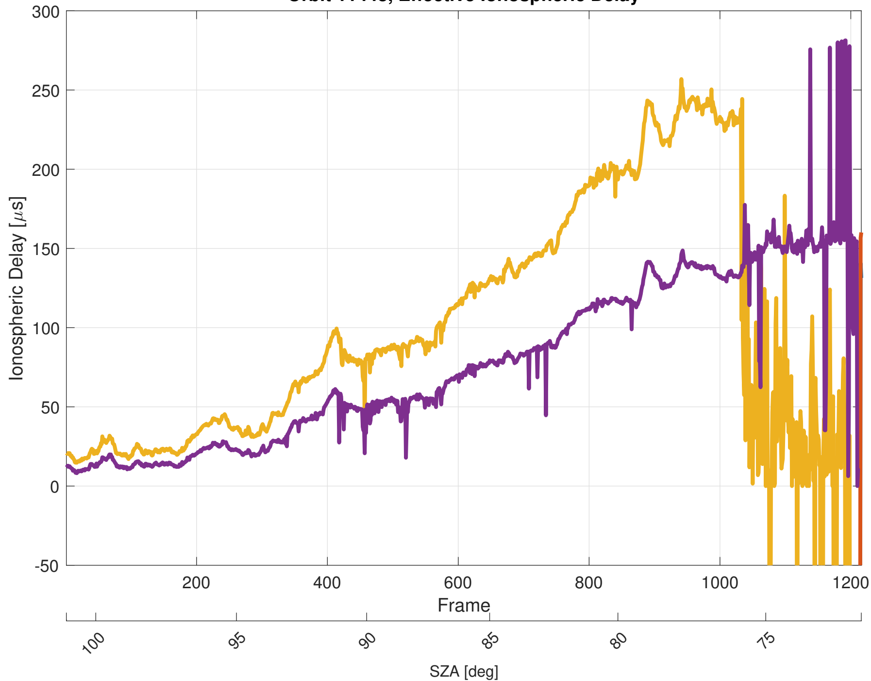
Orbit 11448, Effective Ionospheric Delay
